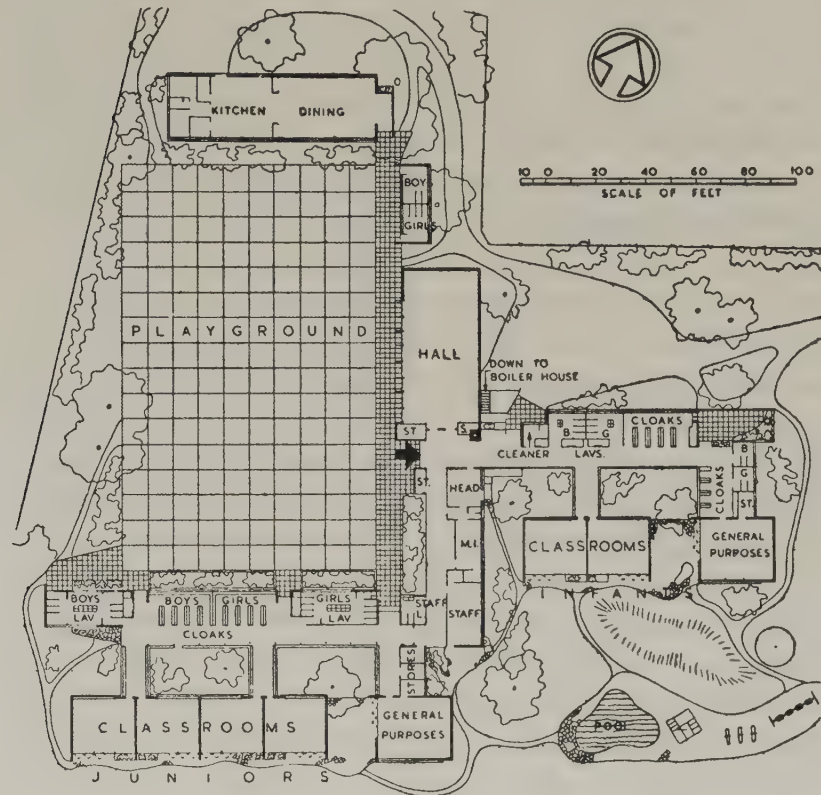
Fig.1 Denis Clarke-Hall, plan of the Junior and Infant School, Ormesby, Yorkshire. Credit: Denis Clarke-Hall, plan published in John Summerson, Heavenly Mansions and Other Essays on Architecture (New York: W. W. Norton & Company, 1963).
