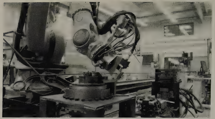
A robot bender cold-forms the steel rods
