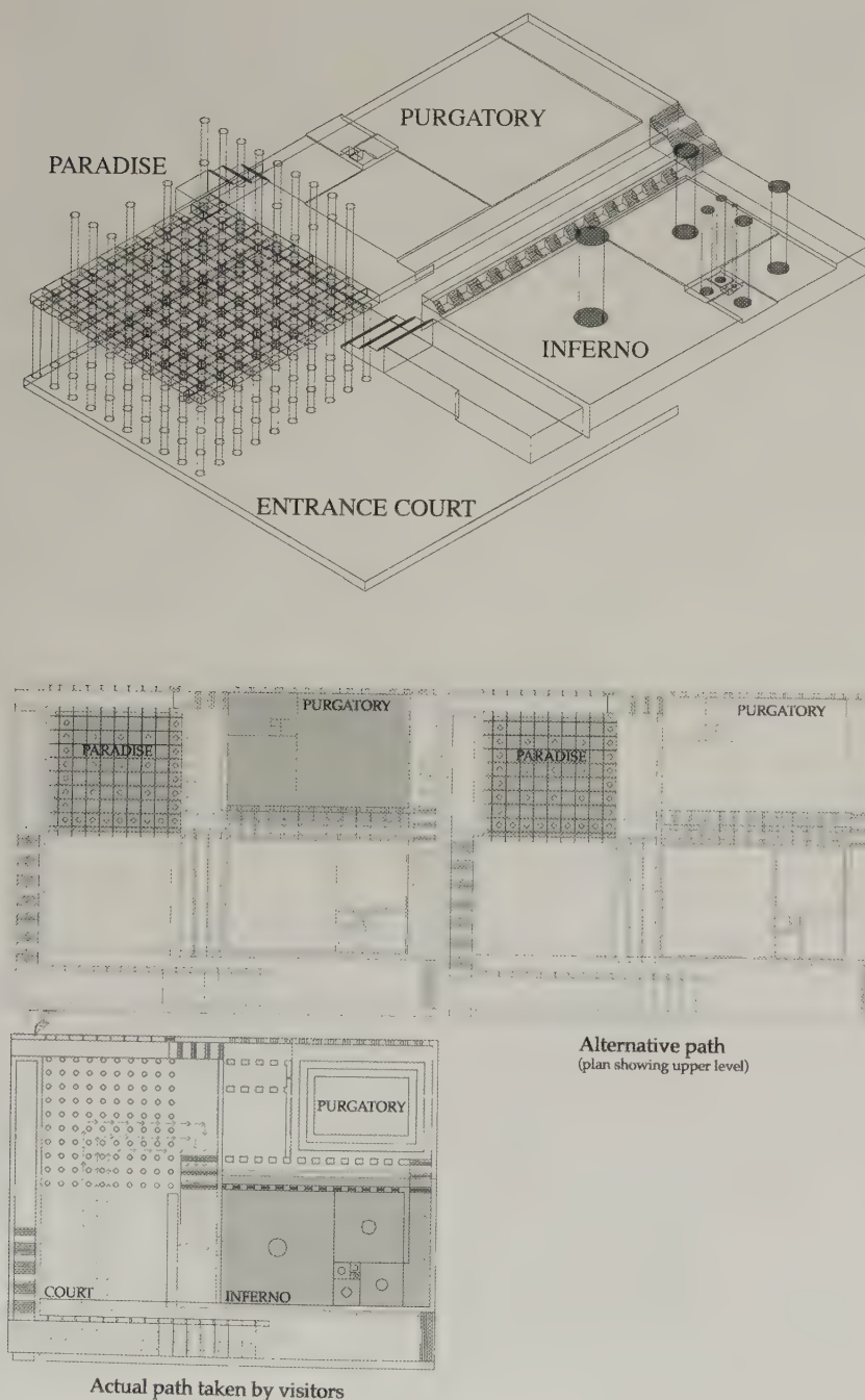
Figs. 8a, 8b Danteum project (Giuseppe Terragni and Pietro Lingeri, 1938). Axonometric drawing and plans by the author
