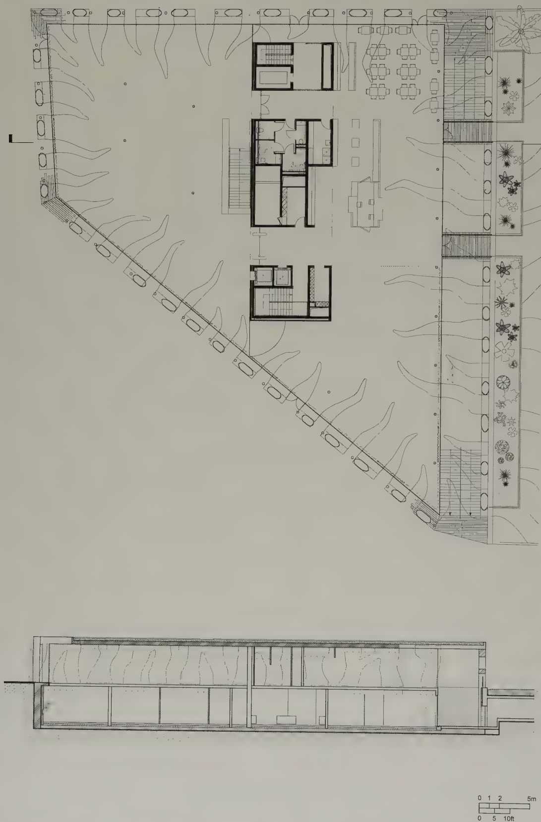
Ground floor plan and section. Credit: Agence Rudy Ricciotti
