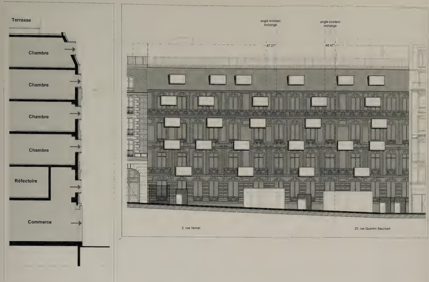
Sectional diagram and unfolded elevation. Credit: Maison Edouard François
