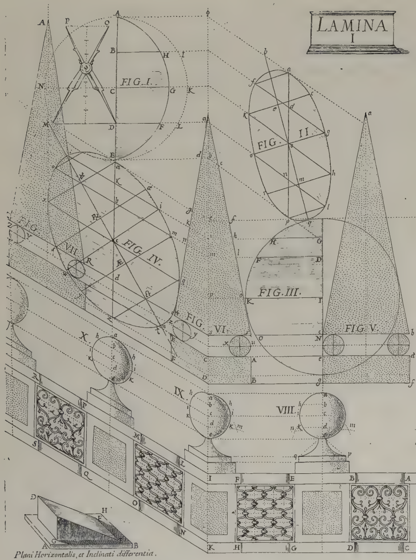
Fig. 17 Juan Caramuel de Lobkowitz, image of balustrade distortion from Architectura Civil Recta, y Obliqua (Vigevano, 1678)
