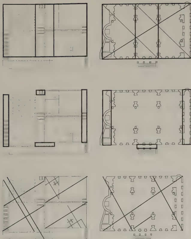
Fig. 9 Golden section rectangle proportioning in comparison with Basilica of Maxentius after Thomas Schumacher
