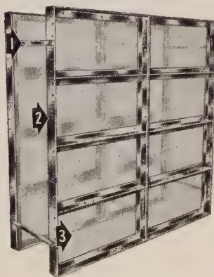
1. Ties spread, lock UNI-FORMS into a form with automatically accurate wall thickness.
