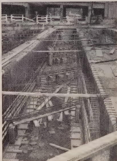
SUPPLEMENTARY REINFORCING STEEL in position around tendons, and bridge girder.
