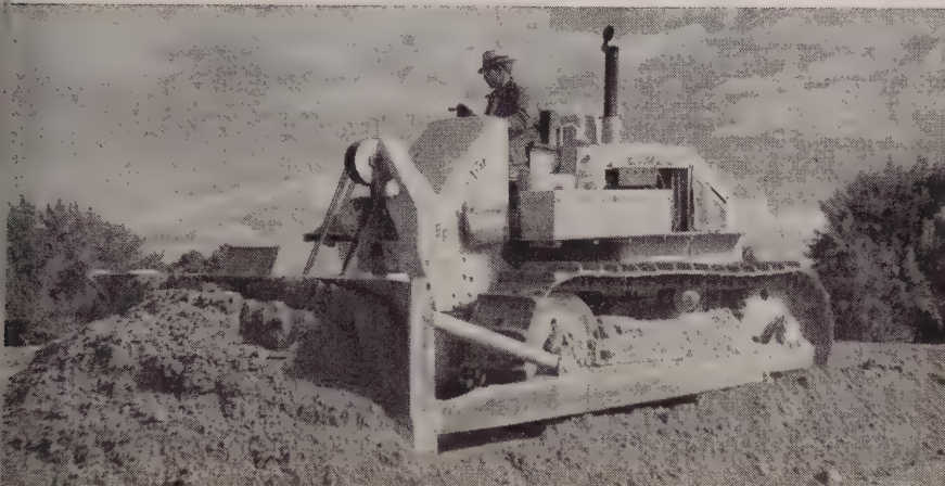
ON THE FILL material is spread by two tractors with dozers: an IH TD 24 and an Eimco model 106 shown here. Front location gives operator good visibility, an asset in tight spots.
