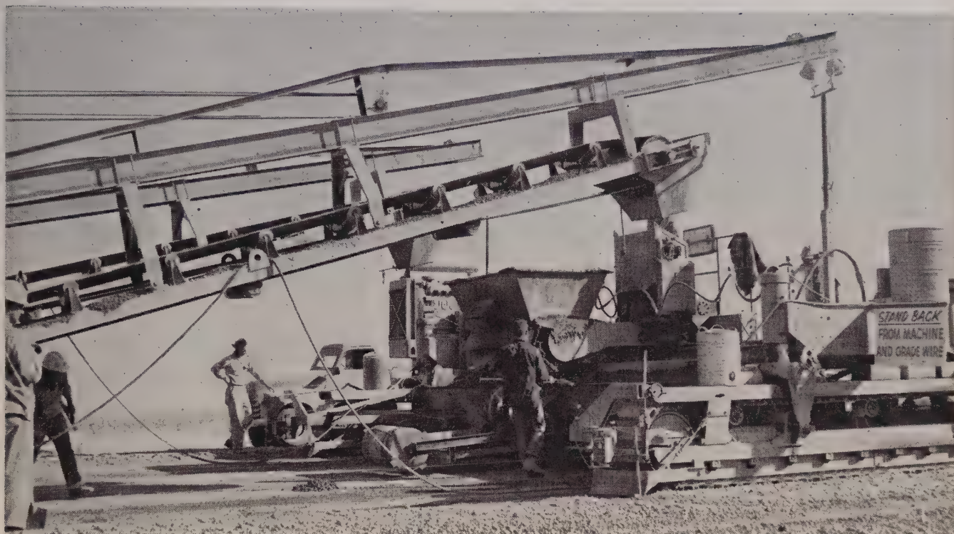
CRAWLER assemblies carry slip-form along grade at 7 fpm. guided by grade wires at either side. Belts from pavers replace conventional
