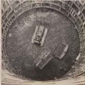
40 ft dia 180' deep surge tank excavated by drilling the granite rock in 5 ft deep rounds using Brunner & Lay Rok-Bits. An average of 90 eight yd buckets of rock removed each day.
