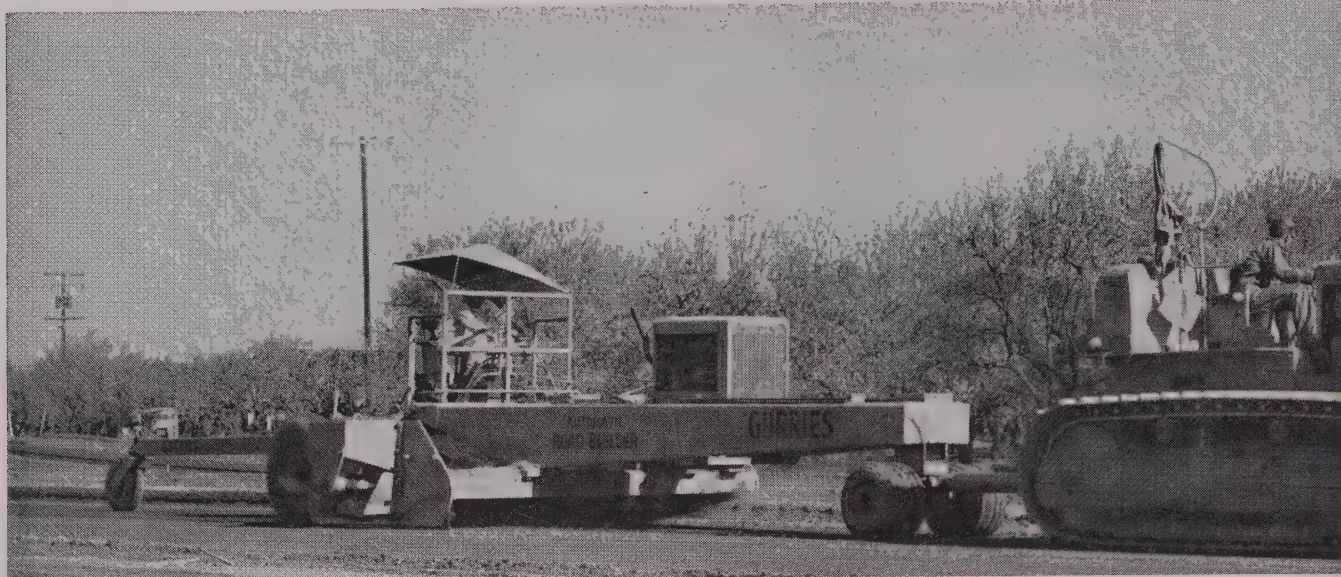
GURRIES "Road Builder" grades a 13-ft. lane, holds grade and cross slope with automatic hydraulic controls. Machine has 44-ft. length
