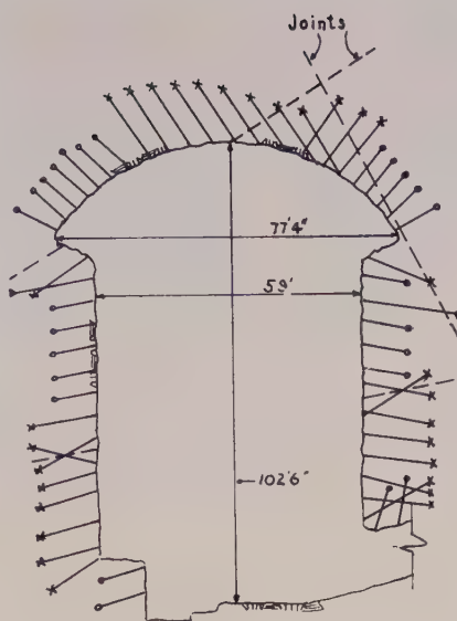
PATTERN for rock bolting during excavation of a large underground hydro power plant in Australia. Spacing was on a 5 x 5-ft. pattern. Note 77-ft. arch span and 102-ft. height.
