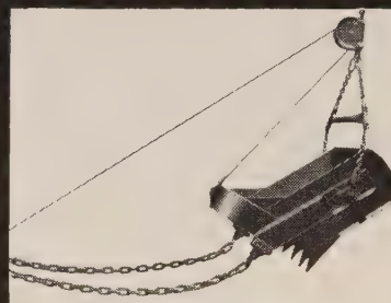
MEDIUM WEIGHT DRAGLINE, Type M , balanced for easy digging and full payload.
