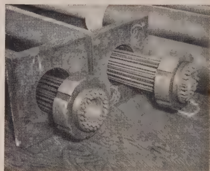
40-WIRE ASSEMBLIES in flexible conduit before placement—showing moveable anchor head, lock nut, base plate, and trumpet encasing last few feet of flexible conduit.
