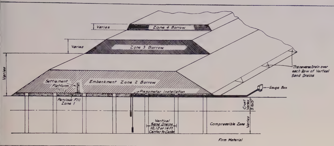
SCHEMATIC DIAGRAM OF SAND-DRAIN EMBANKMENT
