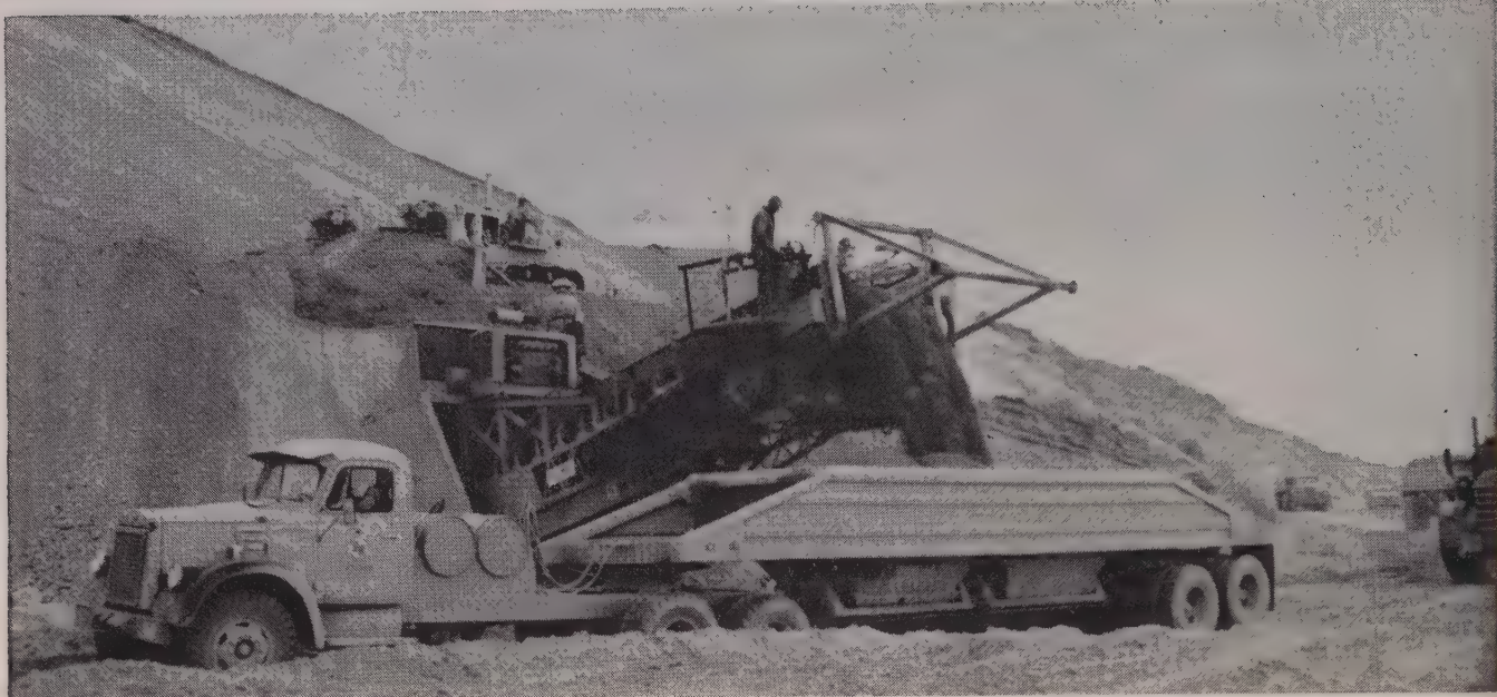
LOADING OPERATION is fast, averaging 8,000 cu. yd. per day through belt loader. Two to four D8 Cats keep the Kolman belt hopper full. Contractor has 16 rigs making 15-min. round trip with fill material. Ten are Cook Bros. trailers, 20-ton capacity, pulled by IH tractors.
