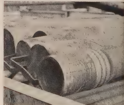
DRILLING joint faced with tungsten carbide
