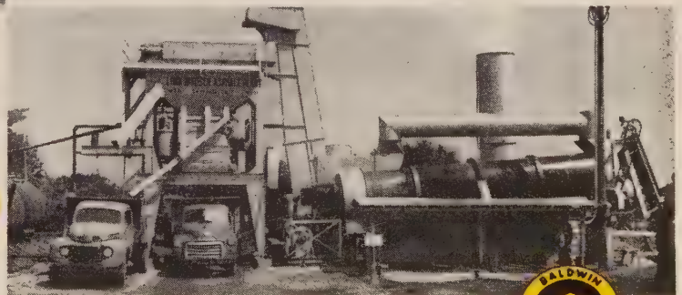
THE LITTLE MONSTER ®...this complete asphalt mixing plant on wheels is designed for fast-moving, fast set-up and substantial daily production. Plant shown is owned by a State Highway Department. It is complete including two MADSEN 32" x 10' Dryers, a MADSEN 2-compartment portable feed bunker and dual cold stone elevators. Mixer unloading skip loads asphalt into trucks. Plant is rated at 30 T.P.H. on a one-minute mixing cycle.
