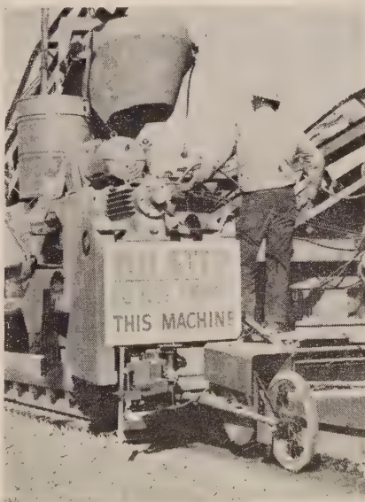
BICYCLE wheel controls interval between transverse joints. Hinged control fork swings past grade stake.
