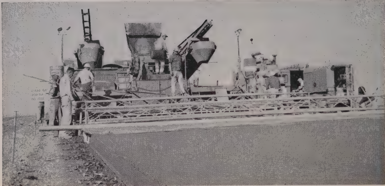
EXPOSED edge of fresh slab placed with slip-form. Unit tows 35-ft. V-float with side forms. Grade stakes at left. Electrically powered
