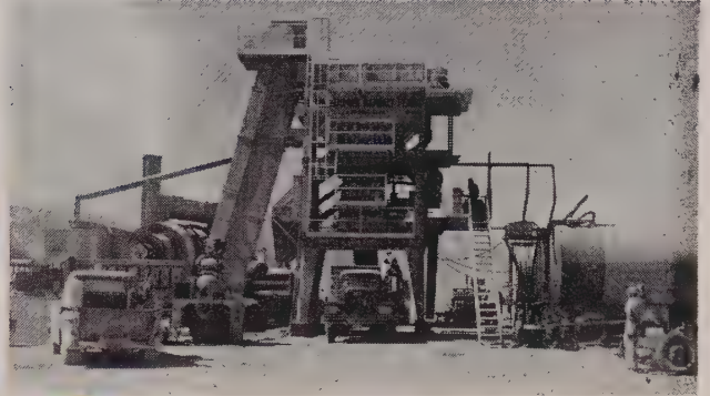
MADSEN MODEL 481 ASPHALT PLANT ...the industry's outstanding batch capacity asphalt plant, built in 4000 lb., 5000 lb. and 6000 lb. capacities. Factory-matched unit sections assure quick field erection. Plant features faster mixing, exclusive bin design for more uniform aggregate withdrawal, roll-away weigh-box for quick, easy servicing and maintenance, and finger-tip control of weighing and mixing operations. (Fully automatic operation is optional.) Capacities up to 300 T.P.H.
