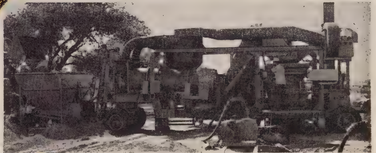
THE LITTLE MONSTER ®...this complete asphalt mixing plant on wheels is designed for fast-moving, fast set-up and substantial daily production. Plant shown is owned by a State Highway Department. It is complete including two MADSEN 32" x 10' Dryers, a MADSEN 2-compartment portable feed bunker and dual cold stone elevators. Mixer unloading skip loads asphalt into trucks. Plant is rated at 30 T.P.H. on a one-minute mixing cycle.
