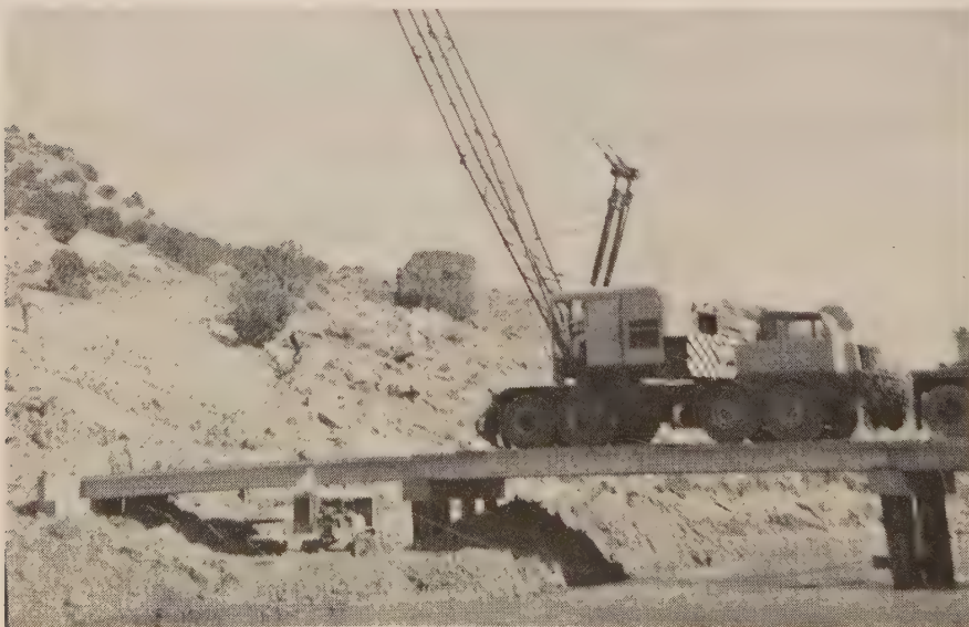
NEW BRIDGE supports 42-ton carrier crane and 40-ton trailer load as final span is placed. Each span made up of nine prestressed girder-deck members.
