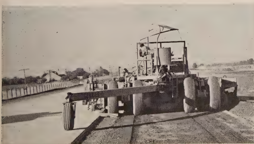
SHOULDERS graded for hot-mix application by Gurries machine. Guide wheel on slab is base for automatic cross slope control. Trailing wheel is not used in shoulder grading work.
