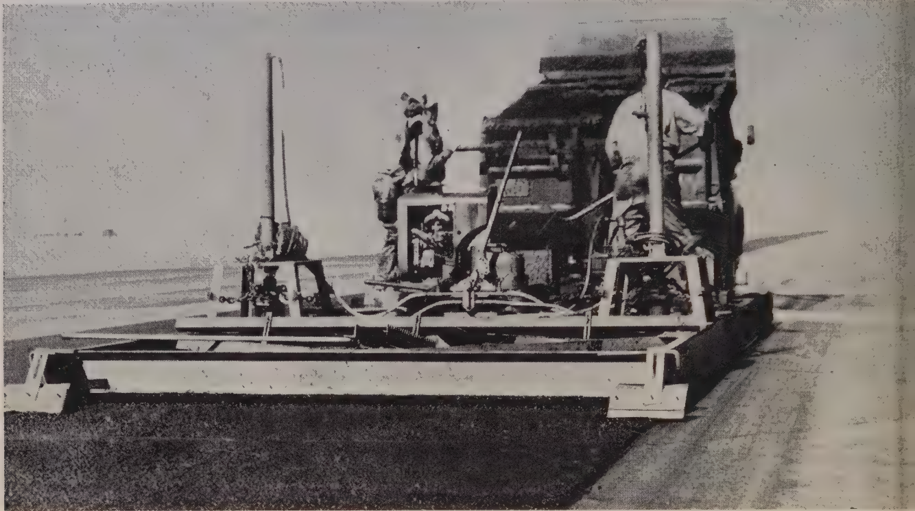
THIS sturdily-constructed spreader-box was used to apply both the Bitumuls asphaltic concrete and the slurry seal used in beefing-up the main runway at Mountain Home Air Force Base. The machine is spreading the overlay, and was later used to spread the seal.
