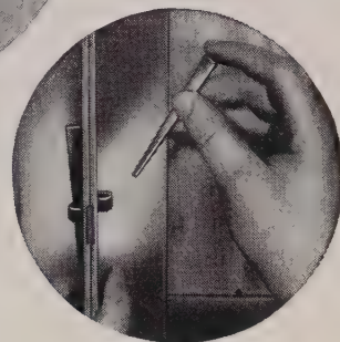
3. Next UNI-FORM Panel is placed in position. Tie Loop automatically enters square tie hole. Key is dropped in—assembly is complete. NO COMING BACK TO "FISH" TIES.
