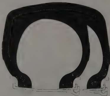
COMPARISON of conventional and wide-base tires shows the increase in contact area. Conventional tire is a 24.00 on a 17.00-3½ rim, and wide base is a 29.50 on a 25.00-3½ rim.
