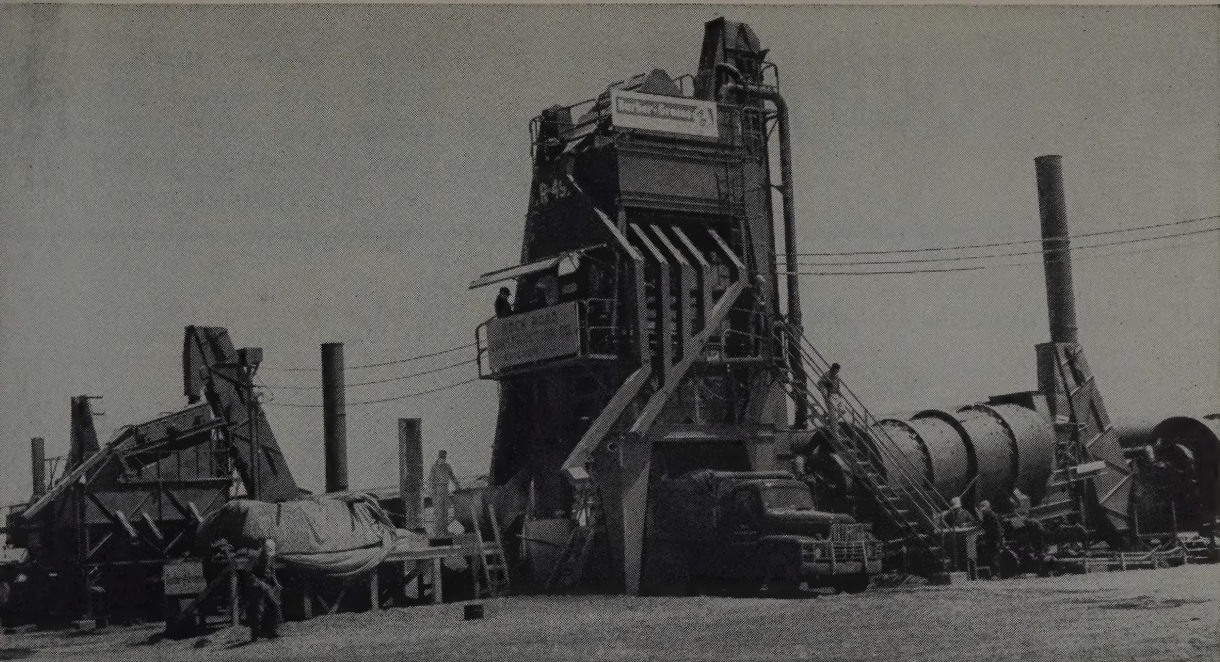
At left is the Barber-Greene Continuous Plant; at right is the BatchOmatic. Together these plants produced all asphalt tonnage on the test road. Both proved their ability to meet abnormally rigid specifications.
