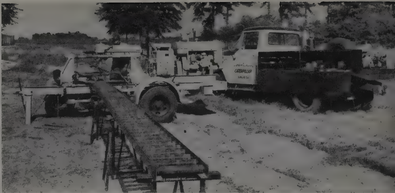
PORTABLE hydraulic track presses, such as the one shown here, greatly reduce the amount of time and trouble needed to turn pins and bushings. Rotating pins and bushings doubles their life. They should never be lubricated.
