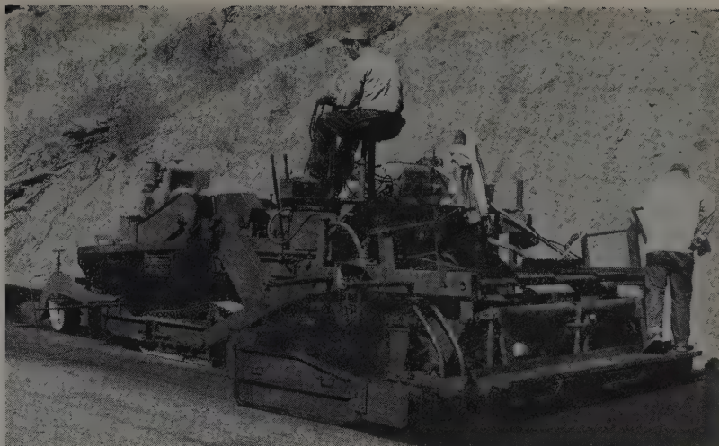
From the windrow, the Pioneer Vibromatic paver is placing a 1¾-in. leveling course 14 ft. wide. It was followed by a surface course of the same depth.
