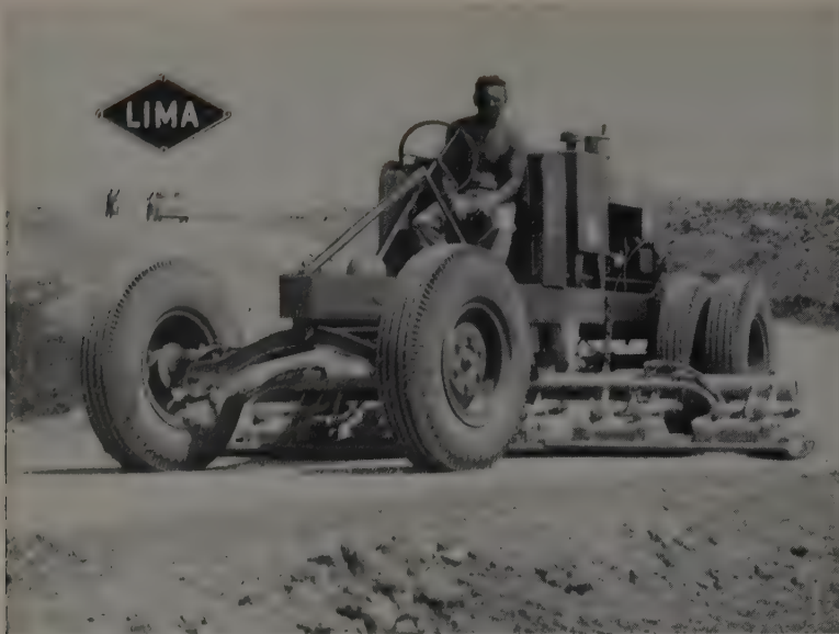
One of six Lima Roadpackers on Illinois East-West Tollway Project pauses here for the photographer during vibratory compaction operations on access road.
