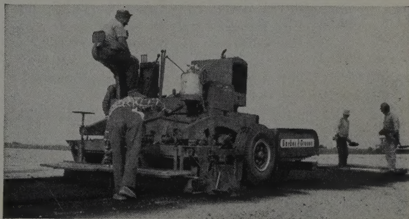
Paving on crawlers and traveling on rubber, the new Barber-Greene Model 873 Finisher paved all the test road's 6' asphalt shoulders in four days—at 64 different locations.
