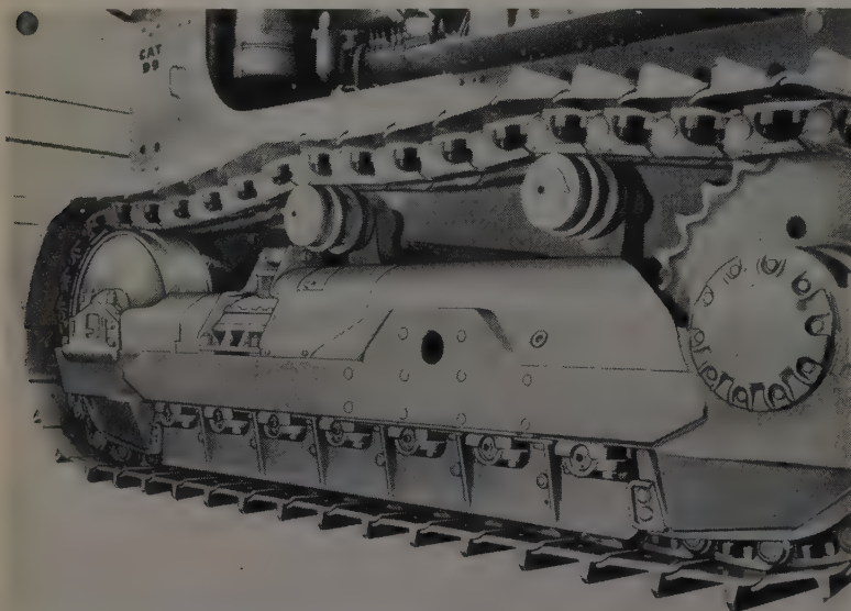
TRACK ROLLER GUARDS are important in rock work. They protect the component parts of the track from unnecessary abrasion and impact damage. Proper shoes and grousers are important.
