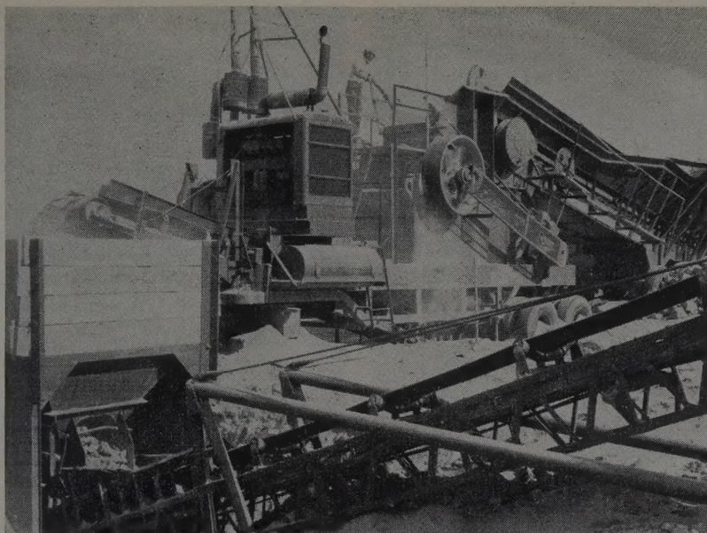
FROM THIS primary crusher the material moves by 30-in. belt to a second portable reduction unit which has a jaw crusher and scalping screen. The set-up was designed to produce all required material: base course, leveling course, aggregate for the plant-mix surfacing and chips.
