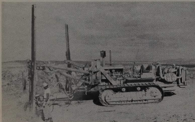
IN THE QUARRY mobile equipment uses 20-ft. steel with tungsten carbide drill bits to put down holes in the tough malpais. Spacing was at 5 ft. and powder averaged 1 lb. per yd. in place.
