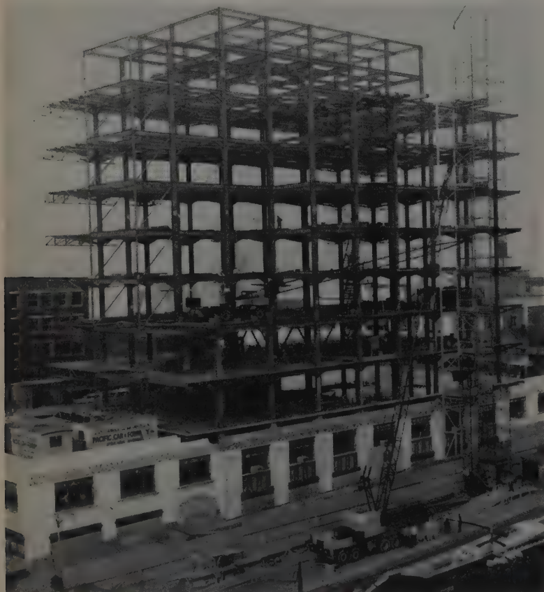
ALL-WELDED STEEL construction features the seven-story addition to City Light office building in Seattle. At a cost of $3,700,000 the Utility will have the building ready for occupancy by late fall. The exterior walls will be lightweight aluminum spandrels and green-tinted glass. Sash will be fixed and the building air conditioned throughout. Note the cantilever of the floors, which extend out 12 ft. aided by the light weight of the walls.
