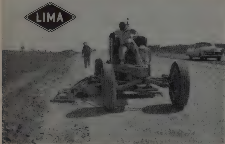
Lima Roadpacker owned by N. H. Garman & Bros., Inc., Reading, Pa. Shown working on highway widening job on U. S. 22, near Harrisburg, Pa. Work involved widening outer strips of 4-lane highway by 33-in. The trench, 9-in. deep, was first lined with a 1 1/2-in. cushion course of screenings. The entire 9-in. lift of 4-in. stone was then tightly keyed in two passes of the Roadpacker. It took only two applications of dry screenings to fill the voids.
