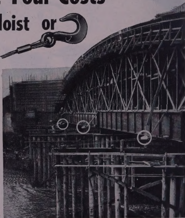
75-ton false work moved 26½ feet horizontally with 5 Griphoists.
