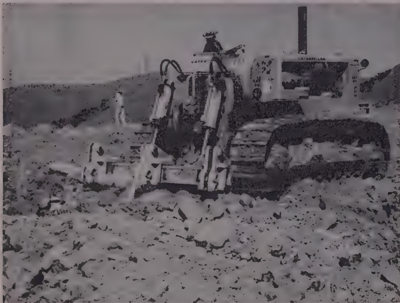
WEIGHT on the teeth and power to pull them is the key in ripper effectiveness. Largest size of modern tractors provides these elements making possible major advance in ripping.
