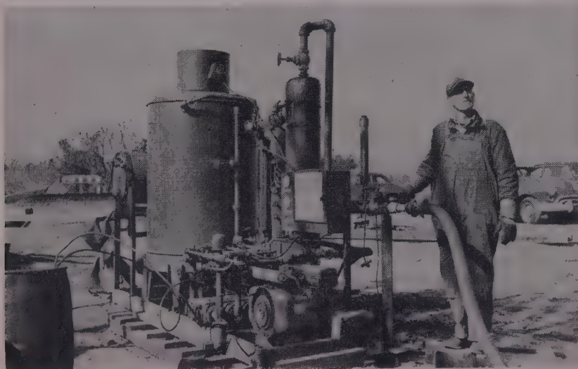
STEAM GENERATOR (McKiernan-Clayton) specially designed to supply power for pile hammers. Full head of steam is generated in less than 3 min., and only in amounts required by the hammer.
