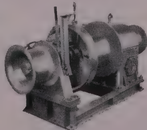
30 H.P. Electric Mooring Winch
