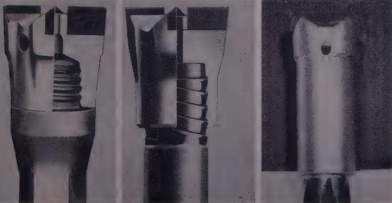
BIT TYPES —Shoulder drive (left), bottom drive (center) and tapered socket connection (right). Each has advantages depending on the type of material and the type of drill.
