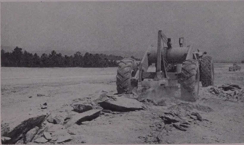
ANOTHER chapter in ripper history is this first unit to be mounted on rubber and pulled by a rubber-tired tractor. Weight is important in keeping the ripper teeth at effective depth.
