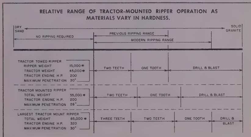
AUTHORITIES on field practice and performance developed this chart to show schematically the ripper range of differing weights and mountings. Limits of range are subject to extreme variation.
