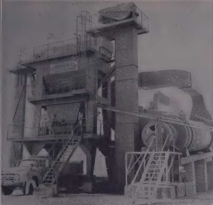
CONTRACTOR DEMANDS have resulted in this semi-portable plant of 6,000-lb. capacity. It can be easily disassembled and transported over state highways with a minimum loss of time.
