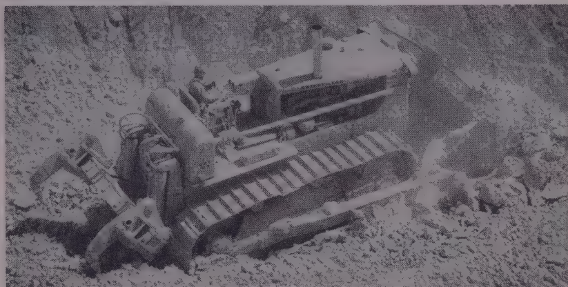
IN THE LIMESTONE quarry of a cement company, this combination bulldozer and tractor-mounted ripper represents the modern unit for moving rock efficiently.
