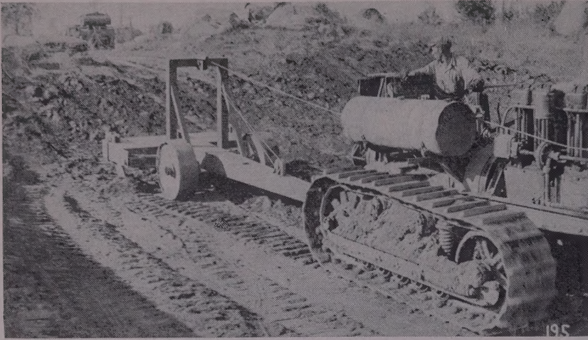
HISTORY was made by this early type of towed ripper. A LeTourneau model of 1933 is shown being pulled by a 60 Caterpillar, gasoline engine powered working in decomposed granite.
