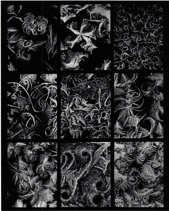
2 Photographs of snow crystals
