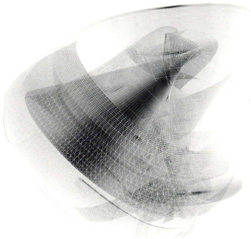
Trefoil, knot with 3 crossings. short elevation.
