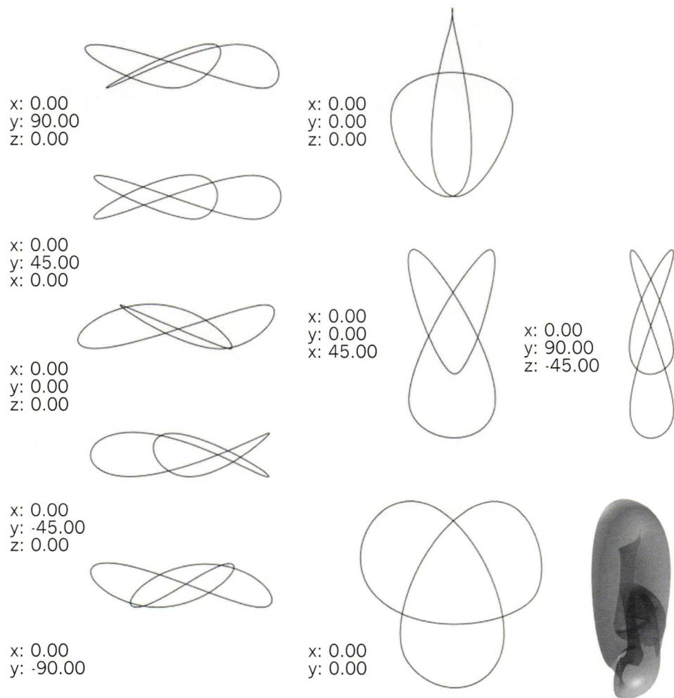
Fig. 1.2: Diagrammatic representations of surface movement based on primitive knot formations.
