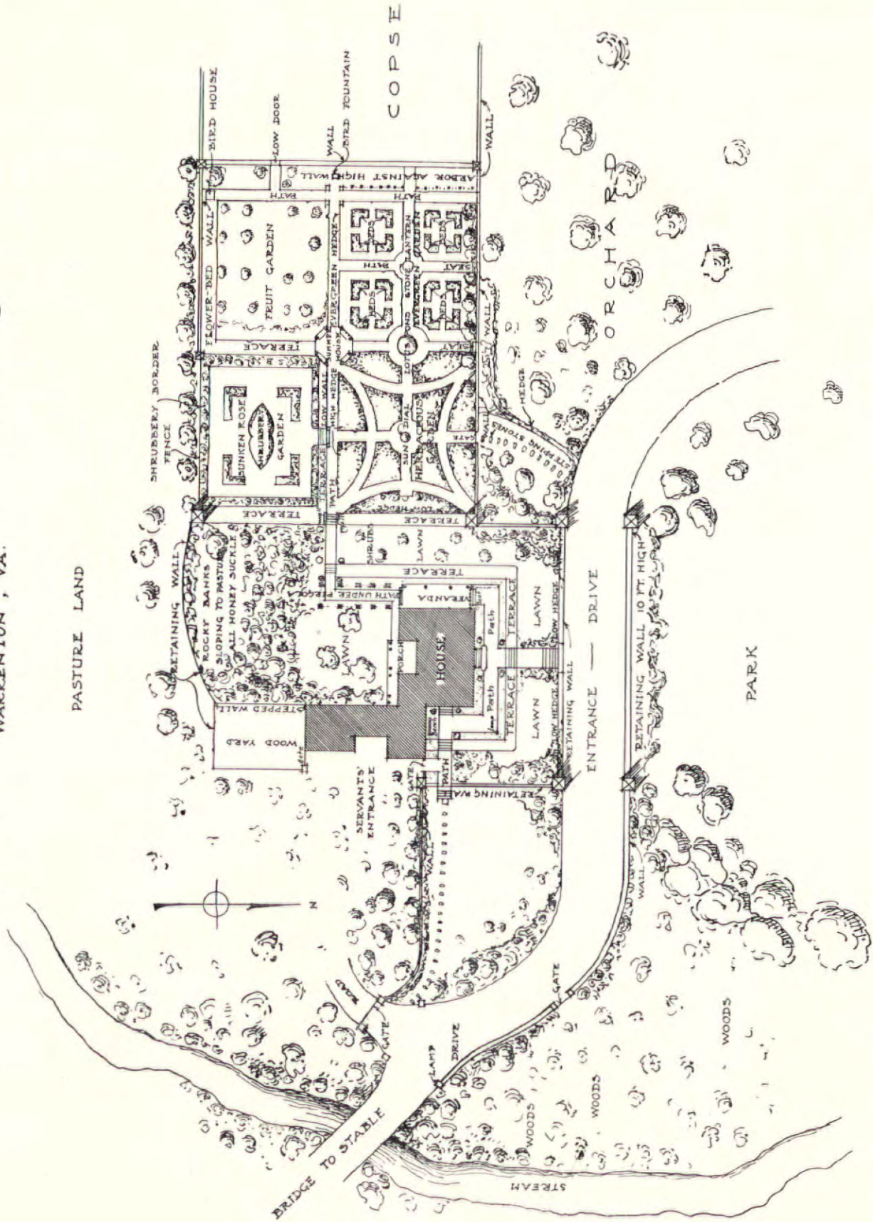
PLAN OF HOUSE AND GROUNDS—"AIRLIE"
