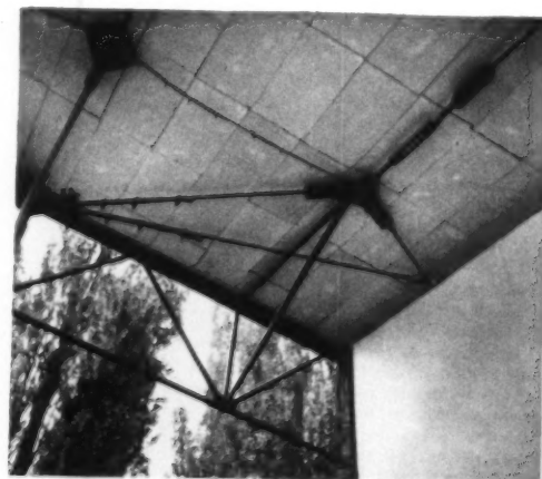
9, detail of roof of Brazilian pavilion showing connection of cables to edge truss.
