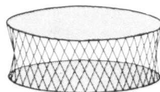
10, diagrams of tension wall of United States pavilion showing, top, plan and elevation of verticals before and after tightening and, right, the finished wall. The curvatures are much exaggerated.
