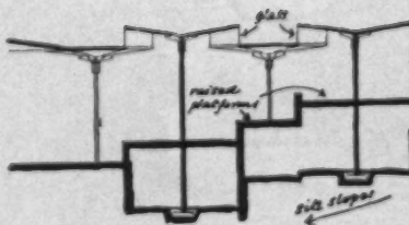
Left, section through the standard umbrella-like roof unit of which the whole structure of the building is composed, and a cross-section through the building showing how these units are stepped up the slope (the length of the stem being varied as necessary) and differ in height to provide clerestory lighting.
