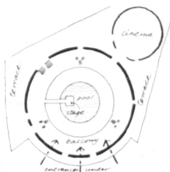
plan of the U.S.A. pavilion. below, structural diagram.
