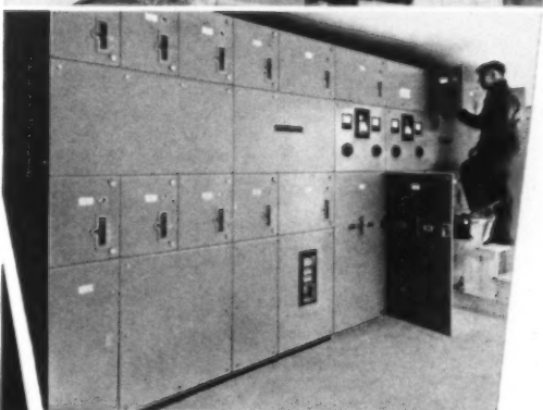
Some of the 'ENGLISH ELECTRIC' equipment being installed in the sub-station
