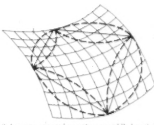
3. two-way opposed curvature or saddle hanging roof.
