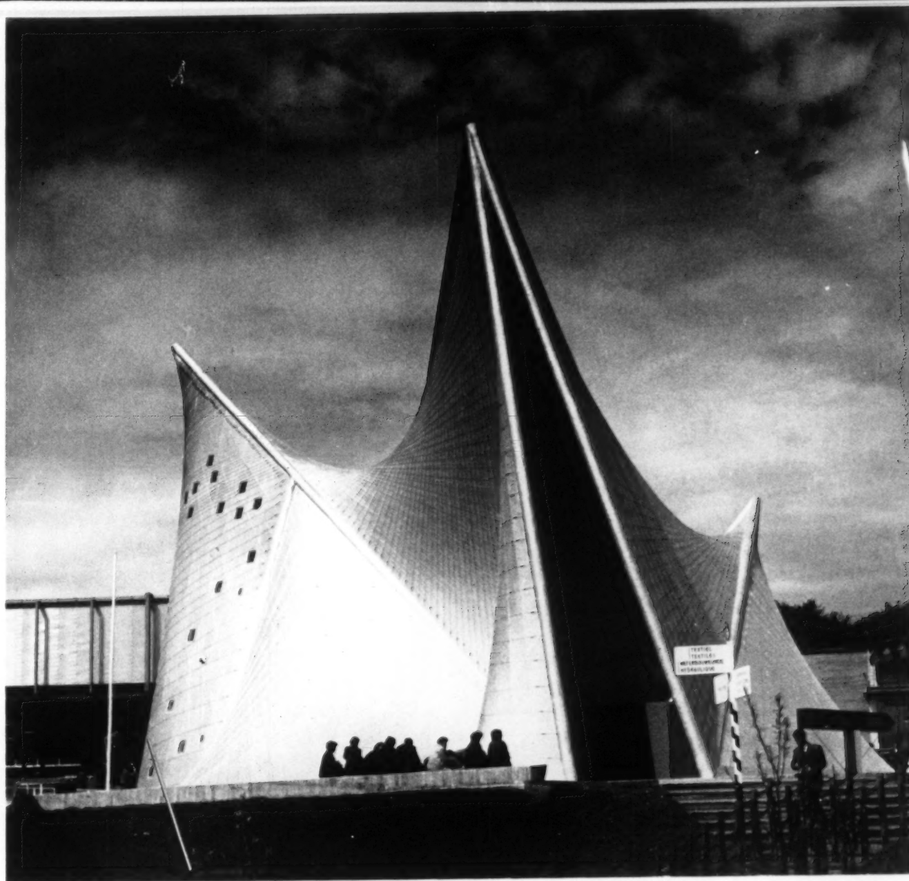
The Philips pavilion, above, housing a poème électronique , adjoins the Netherlands pavilion in the foreign section. It is a reinforced concrete rib structure, with a freely curved plan shape (plan on right), determined by acoustic and lighting requirements, rising to three peaks of 65 ft., 60 ft. and 42 ft. The structure is clothed with a concrete envelope formed of twelve hyperbolic paraboloids and consisting of thin slabs laid on pretensioned cables anchored to the ribs. The inner walls are lined with sound absorbent material and have three hundred loudspeakers built into them. Architect, Le Corbusier; engineer, H. C. Duyster.
