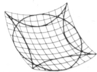
2. double curvature or saucer hanging roof.
