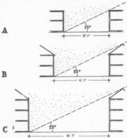
21, application of 25° daylighting angle to three different types of building.
