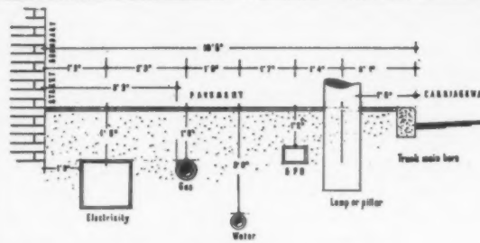
5, three diagrams of underground services: above left, a 10 ft. 6 in. footway; above right, the same services incorporated in a 6 ft. footway, and below, a typical situation at Harlow, where the house-to-road distance is a minimum of 19 feet. Prairie planning becomes automatic before the planner or architect has ever put pencil to paper.
