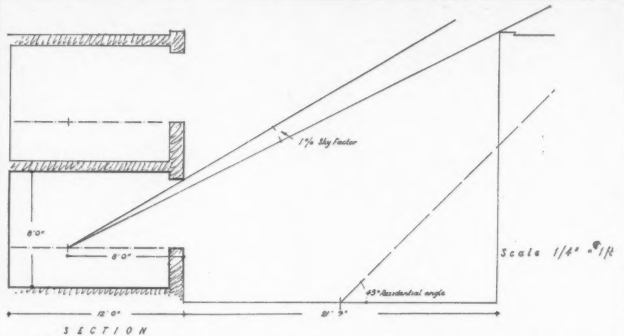
22, minimum spacing of two-storey houses to give recommended daylighting standards—i.e. 1% sky factor 8 ft. inside the room from the window.
