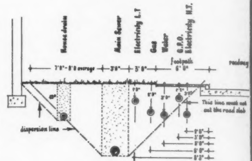
5, three diagrams of underground services: above left, a 10 ft. 6 in. footway; above right, the same services incorporated in a 6 ft. footway, and below, a typical situation at Harlow, where the house-to-road distance is a minimum of 19 feet. Prairie planning becomes automatic before the planner or architect has ever put pencil to paper.
