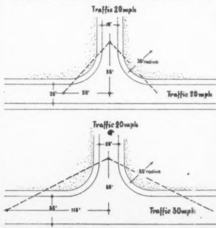
23, the effect on design of junctions of applying standard sight lines for through road traffic travelling at 20 m.p.h. and at 30 m.p.h.
