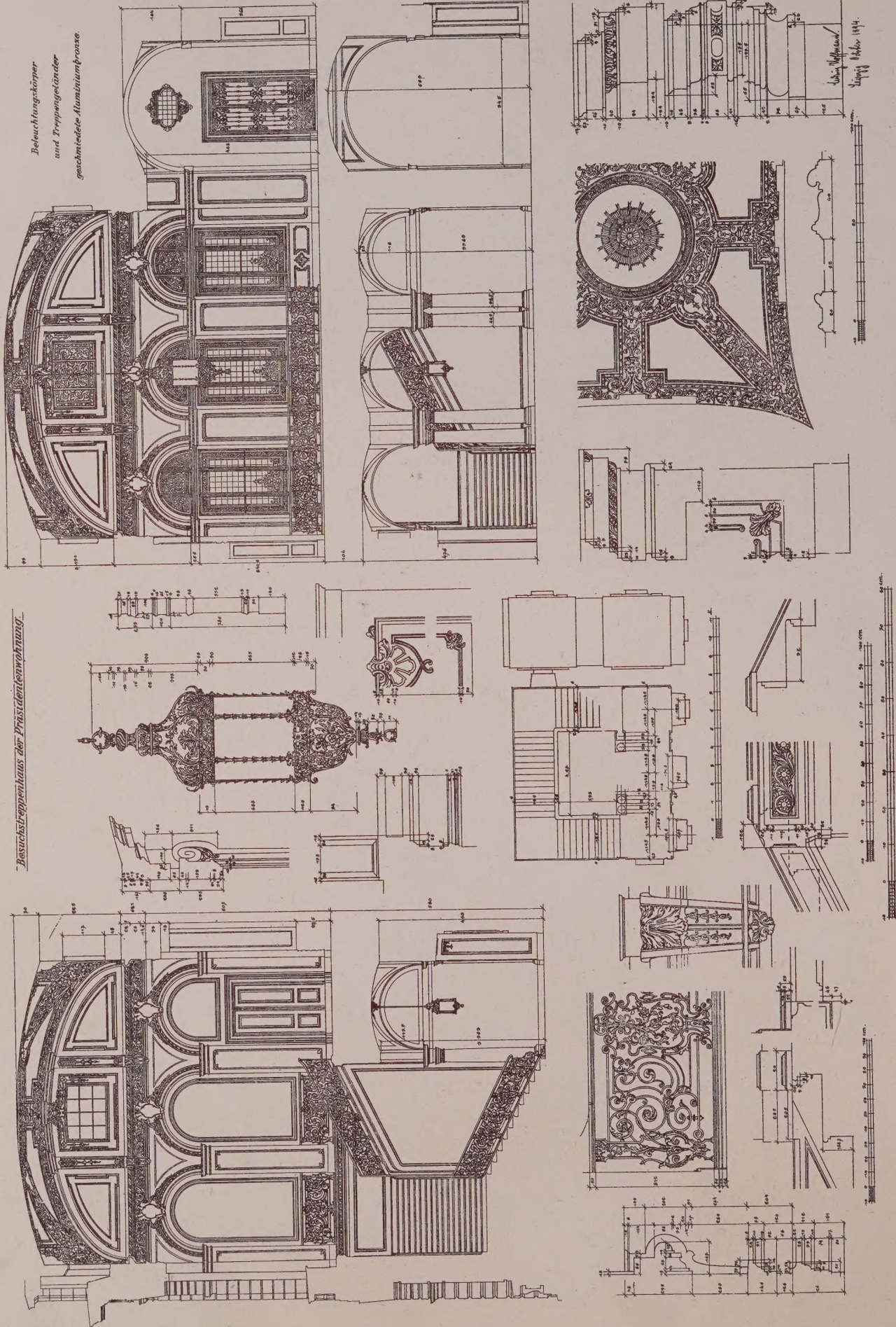
Details of Staircase Hall—President's House,
