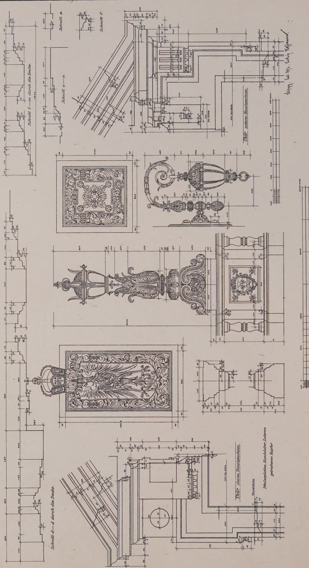
Details of Hall—Imperial Court House, Leipsic
