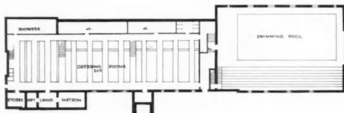
BASEMENT PLAN
