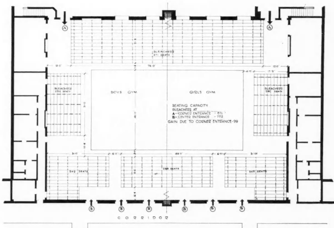
BLEACHER LAYOUT
