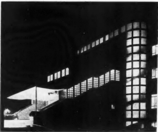
FIG. 7 LUXFER CONCRETE FRAME WINDOWS. AIRPORT IN HAMBURG. DYRSSEN AND AVERHOFF, ARCHITECTS.
