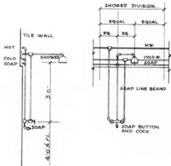
DETAILS OF SHOWER PIPING
