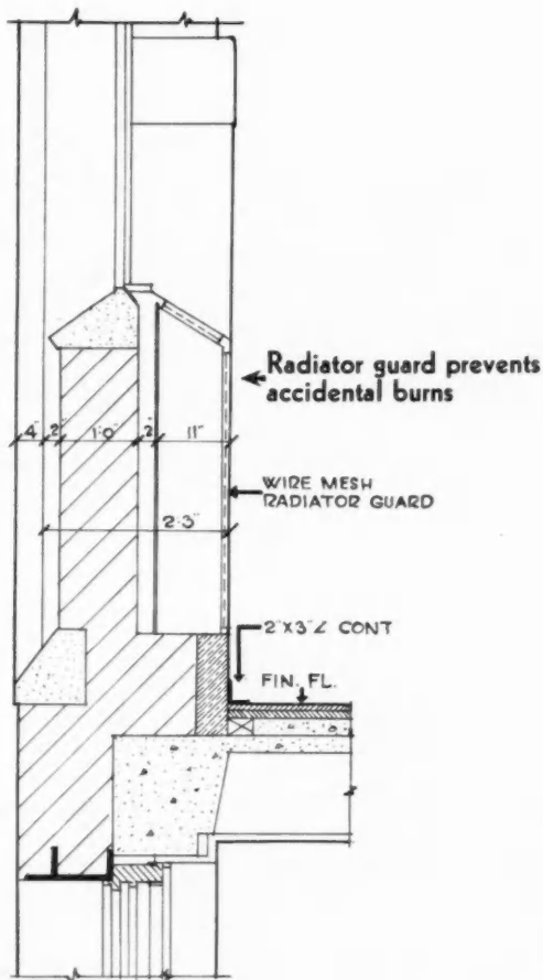
SECTION THROUGH RADIATOR ENCLOSURE
