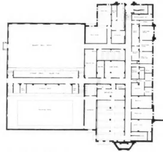
MAIN FLOOR PLAN GYMNASIUM BUILDING
