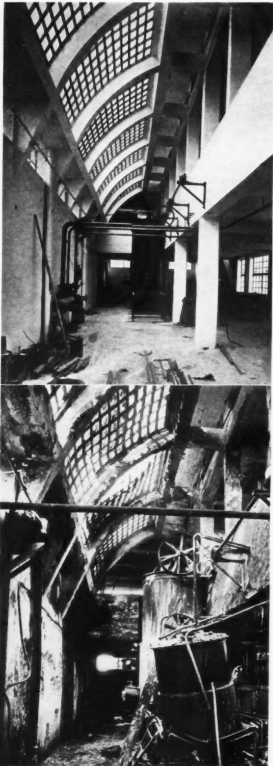
FIG. 1 CURVED LUXFER ROOF CONSTRUCTION FOR OIL REFINERY BEFORE AND AFTER A FIRE. THE TILES BROKE IN THE INTENSE HEAT FROM THE BURNING OIL BUT DID NOT FALL OUT OF THE FRAMES.
