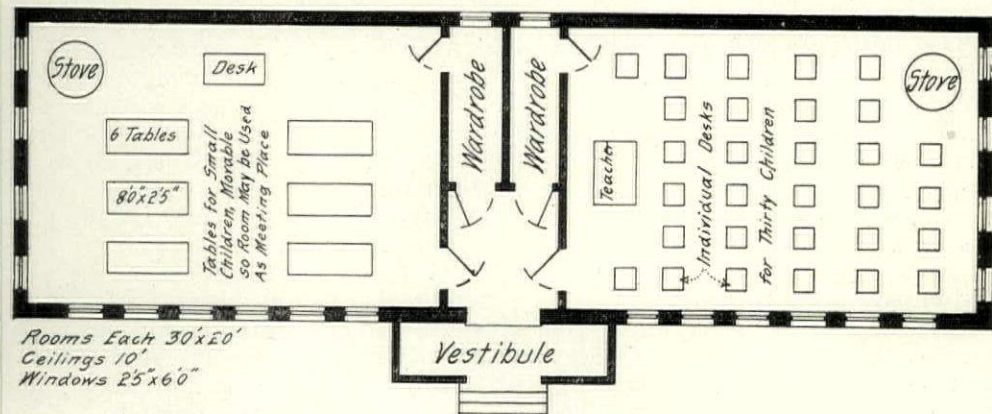
MODEL FLOOR PLAN FOR SMALL SCHOOLHOUSE OF TWO ROOMS.
