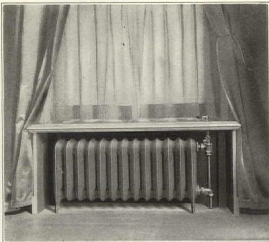
CONCEALED RADIATOR WITH FRONT PANEL REMOVED
