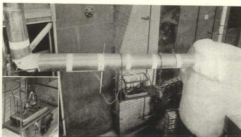
Auxiliary plant for problems on vertical and horizontal ducts, different sizes and shapes of ducts will be tested with different inclinations and lengths of the horizontal duct, insulated and not insulated. The air is heated by steam coils in the large air chamber at the right. The glass encased Wahlen Draft Gauge is shown suspended from the duct with which the draft is measured at various points in the diameter of the duct. An enlarged view of the gauge is shown in the lower left-hand corner. Temperature readings are taken at the base of the vertical duct, at the register and in the duct near the hot air chamber. Velocity measurements are taken at the register with an anemometer.
