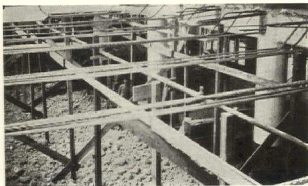
View looking down on first floor. False work for supporting forms already in place.
