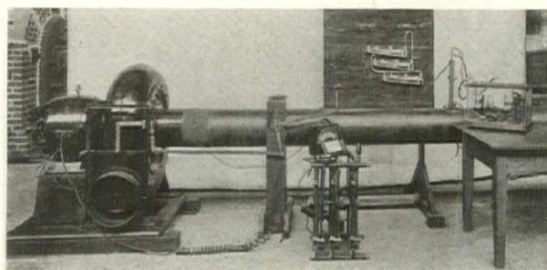
View of a portion of the auxiliary fresh air inlet apparatus. At the left is the exhaust fan attached to the 10 in. pipe connected to the auxiliary inlet shown at the left of the general view of the test plant. The apparatus for regulating the fan and damper is shown. At the table can be seen the Pitot tube for measuring the volume of air passing through the inlet. Readings are taken at various points in the diameter of the 10 in. tube. With velocity conditions at the auxiliary inlet identical with those at the furnace inlet the volume of air passing into the inlets is thus determined.
