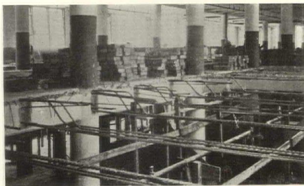
Condition of outer bay after concrete had been removed. Note beam reinforcing rods left in place; also that cases of sheet tin stacked in center panel are located over girders.
