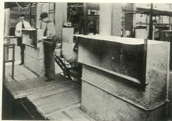
View of the furnace fresh air inlet at the left and the auxiliary fresh air inlet at the right. The anemometer readings are being taken at 24 points on the face of the inlet to the furnace. Identical velocity conditions are established in the auxiliary inlet by means of an induction fan shown in another illustration.
