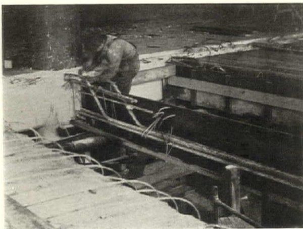
Boxing beam forms around reinforcing rods left in place.
