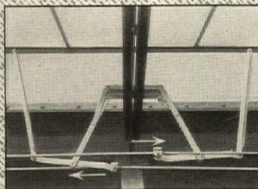
Sash partly open: note arrows.
