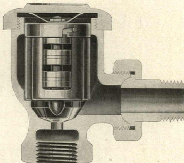
No. 8 Hoffman Return Line Valve
