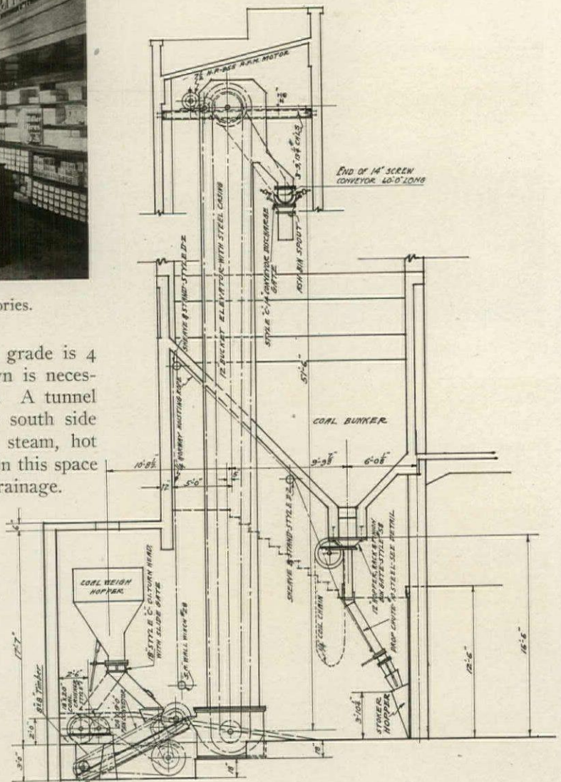
Section through the coal handling plant, showing the weighing hopper with turn-head spout delivering either to a coal crusher or to the elevator boot direct. The 12-in. bucket elevator conveys the coal to a head 52 ft. above the boot and delivers the coal to a 14-in. screw conveyor, 60 ft. long, over the coal bunkers and ash bin. From the reinforced concrete bunkers the coal is spouted to the stoker hoppers.
