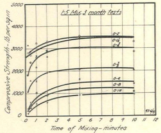
FIG. 14—EFFECT OF TIME OF MIXING ON THE STRENGTH OF CONCRETE
