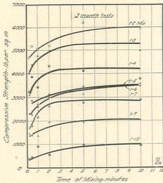
FIG. 12—EFFECT OF TIME OF MIXING ON THE STRENGTH OF CONCRETE
