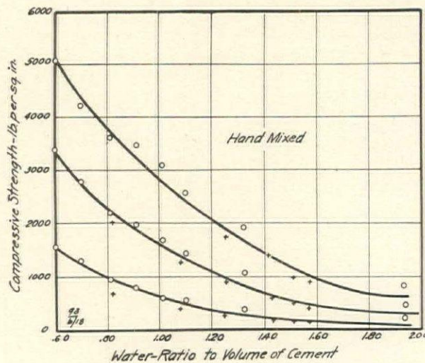
FIG. 17—INFLUENCE OF WATER ON THE STRENGTH OF CONCRETE
