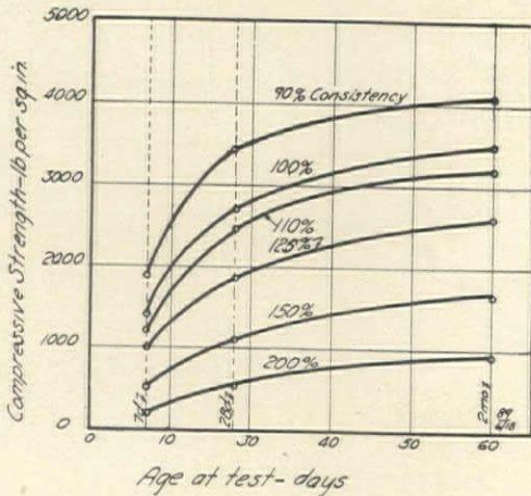
FIG. 10—EFFECT OF AGE ON THE STRENGTH OF CONCRETE
