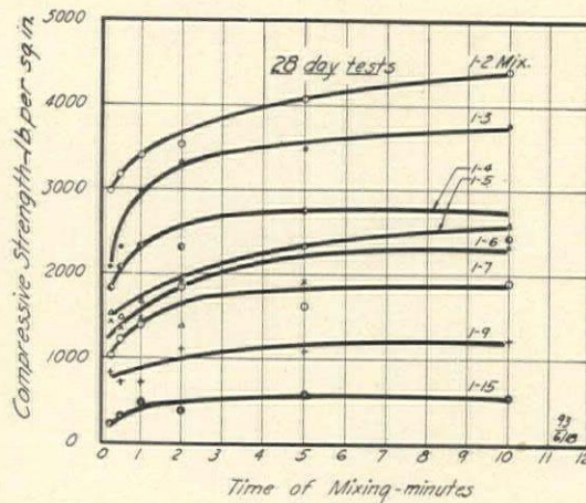
FIG. 11—EFFECT OF TIME OF MIXING ON THE STRENGTH OF CONCRETE
