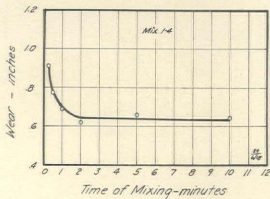
FIG. 6—EFFECT OF TIME OF MIXING ON THE WEAR OF CONCRETE
