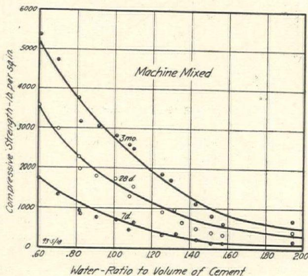
FIG. 16—INFLUENCE OF WATER ON THE STRENGTH OF CONCRETE
