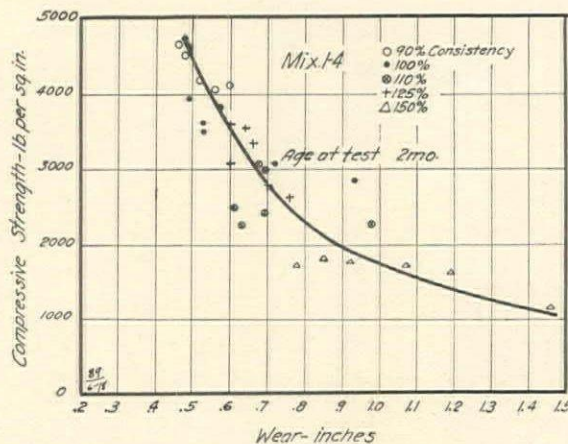
FIG. 8—RELATION BETWEEN STRENGTH AND WEAR OF CONCRETE
