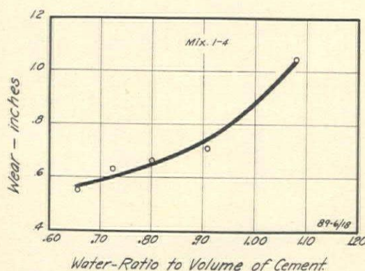
FIG. 7—INFLUENCE OF WATER ON THE WEAR OF CONCRETE
