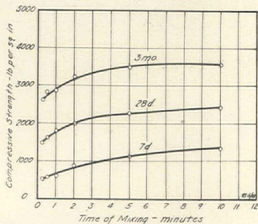
FIG. 15—EFFECT OF TIME OF MIXING ON THE STRENGTH OF CONCRETE
