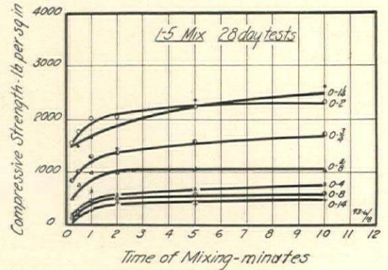
FIG. 13—EFFECT OF TIME OF MIXING ON THE STRENGTH OF CONCRETE
