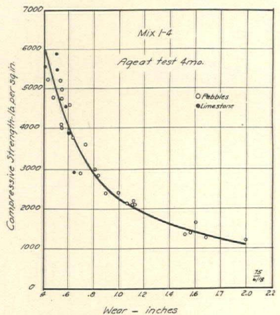
FIG. 9—RELATION BETWEEN STRENGTH AND WEAR OF CONCRETE
