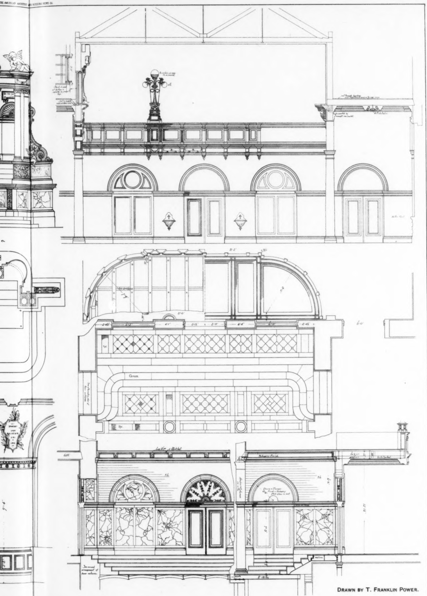
OF THE SACRED HEART, NEWTON CENTRE, MASS. H. MCGINTY ARCHITECT.
