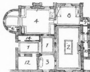
BASEMENT PLAN.
