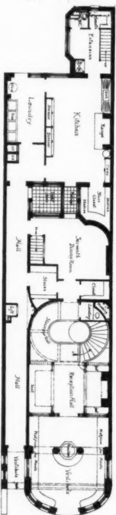
Fourth Floor Plan
