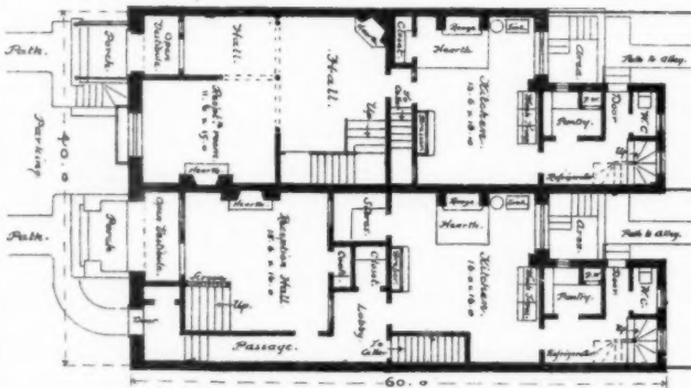
First Story Plan.
