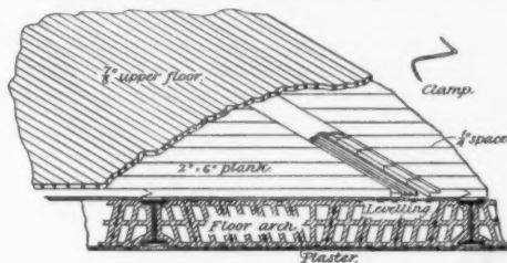
Improved construction.
