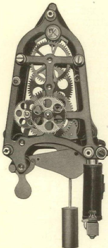
Landis Self-Winding Regulator Movement
