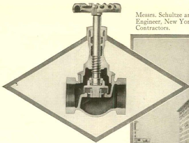
Sectional view of Fig. 106, screwed. Jenkins Standard Bronze Globe Valve.
