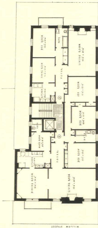
FLOOR PLAN - 7 AND 4 ROOM APARTMENTS
