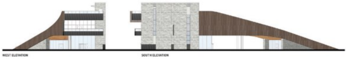
SLEDDING HILL • PAVILION ELEVATIONS © ROSSSETTI
