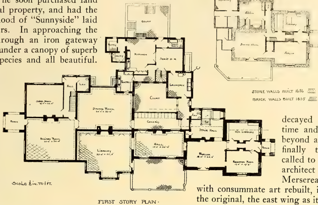
FIRST STORY PLAN.
