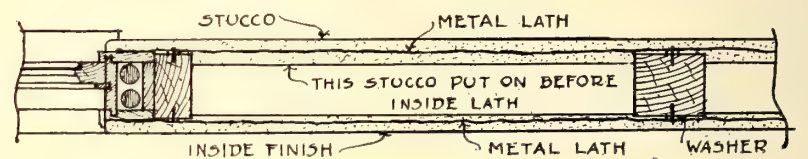
Sketch C, Wall Construction Using Wooden Frame with Stucco on Metal Lath
