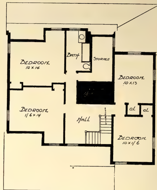
"Naganook": Second Floor Plan
