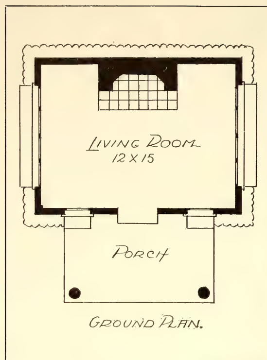
Plan of "Chuckles"
