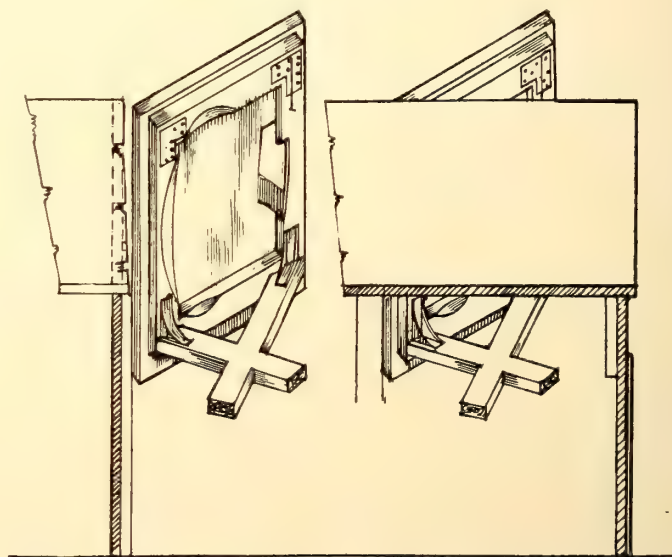
ISOMETRIC PROJECTION REAR VIEW.
