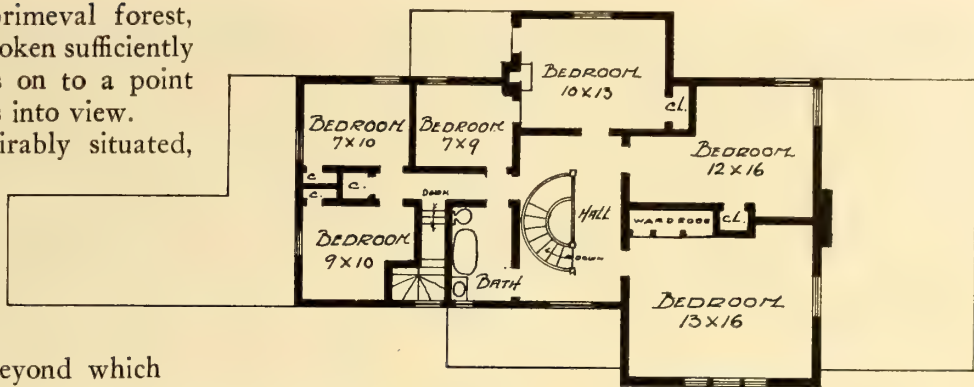
SECOND FLOOR
