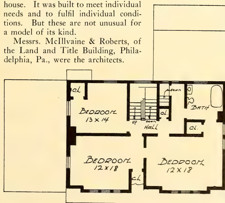
SECOND FLOOR
