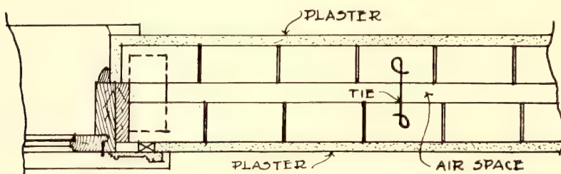
Sketch A, Wall Construction with Rough Brick Plastered
