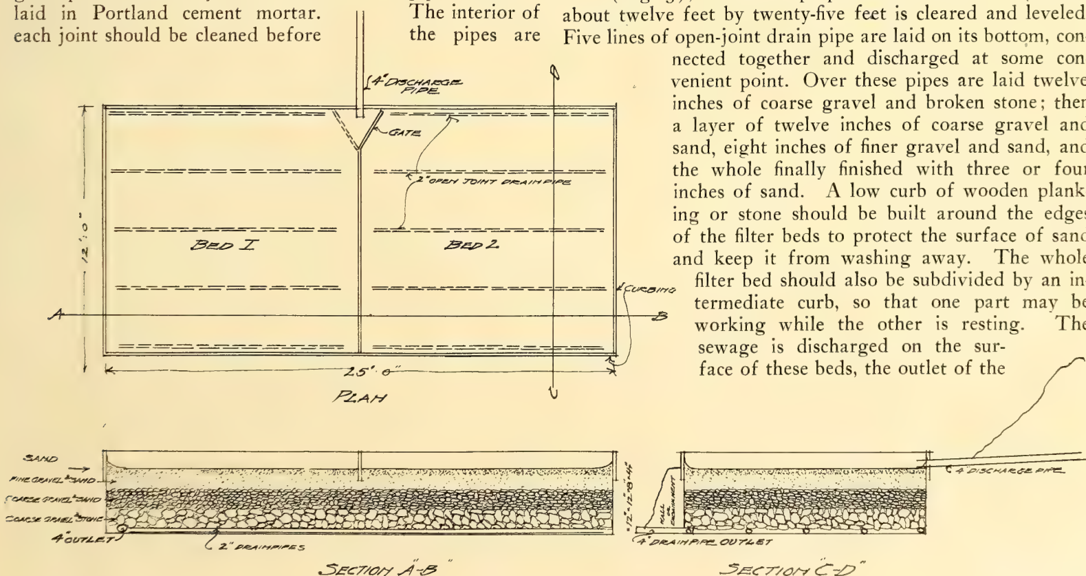
Fig. 3—Plans and Sections of Filtration Beds
