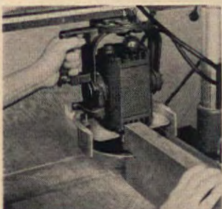
It's a RADIAL SWING SAW . Out-modes any single-purpose swing saw. Does more work and does it differently. Saws at any angle.
