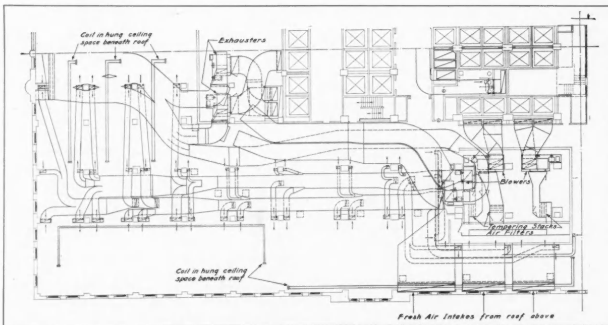
Ventilating System, Northeast Quarter of the Fifth Floor
