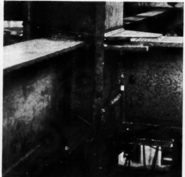
Interior Column Wind-Bracing Detail and Beam Connections
