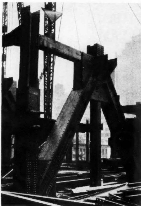
Heavy Truss Over the Lobby, Supporting One of the Tower Columns
