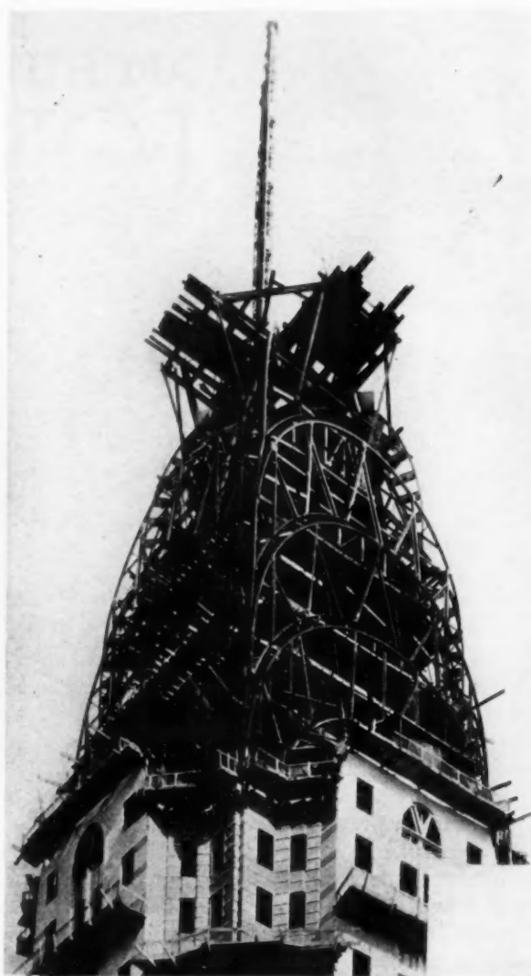
Knickerbocker Complicated Framework of the Dome. Curved Members Were Laid Out on the Mold Loft Floor at the Shipyard
