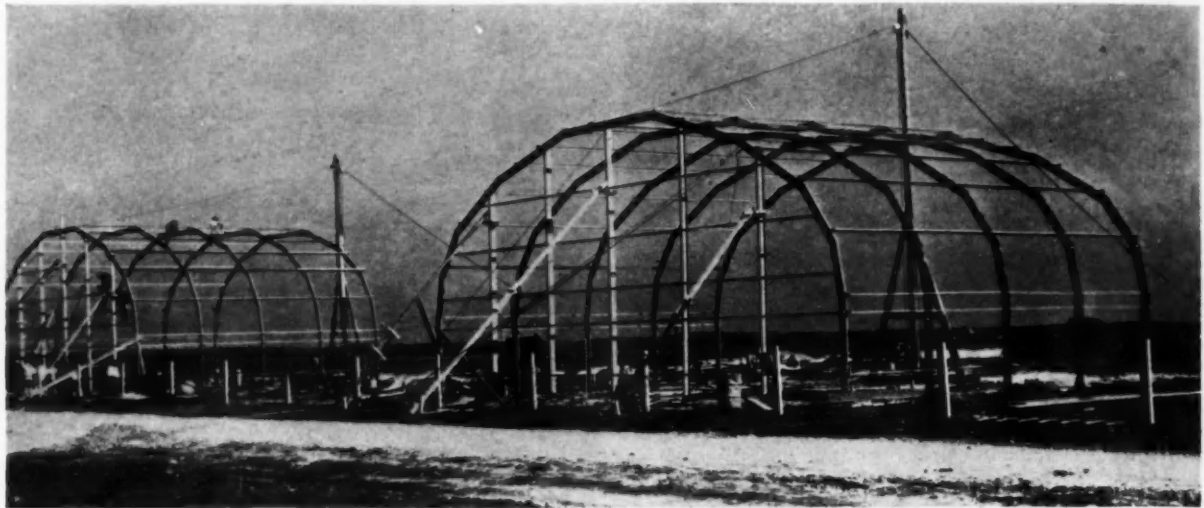
All-Welded Frame for the Houston Airport Hangars. In Background Are Several Motor Trucks with Gasolene Engine-Driven Electric Generators
