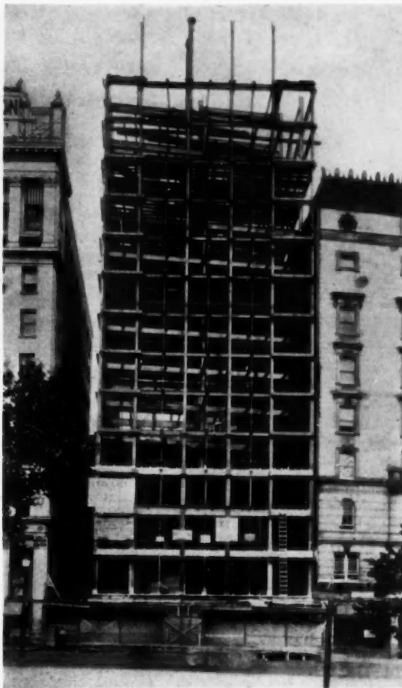
Office Building for the Edison Electric Illuminating Company, Boston, 14 Stories High, 1,400 Tons, Shop-Riveted and Field-Welded
