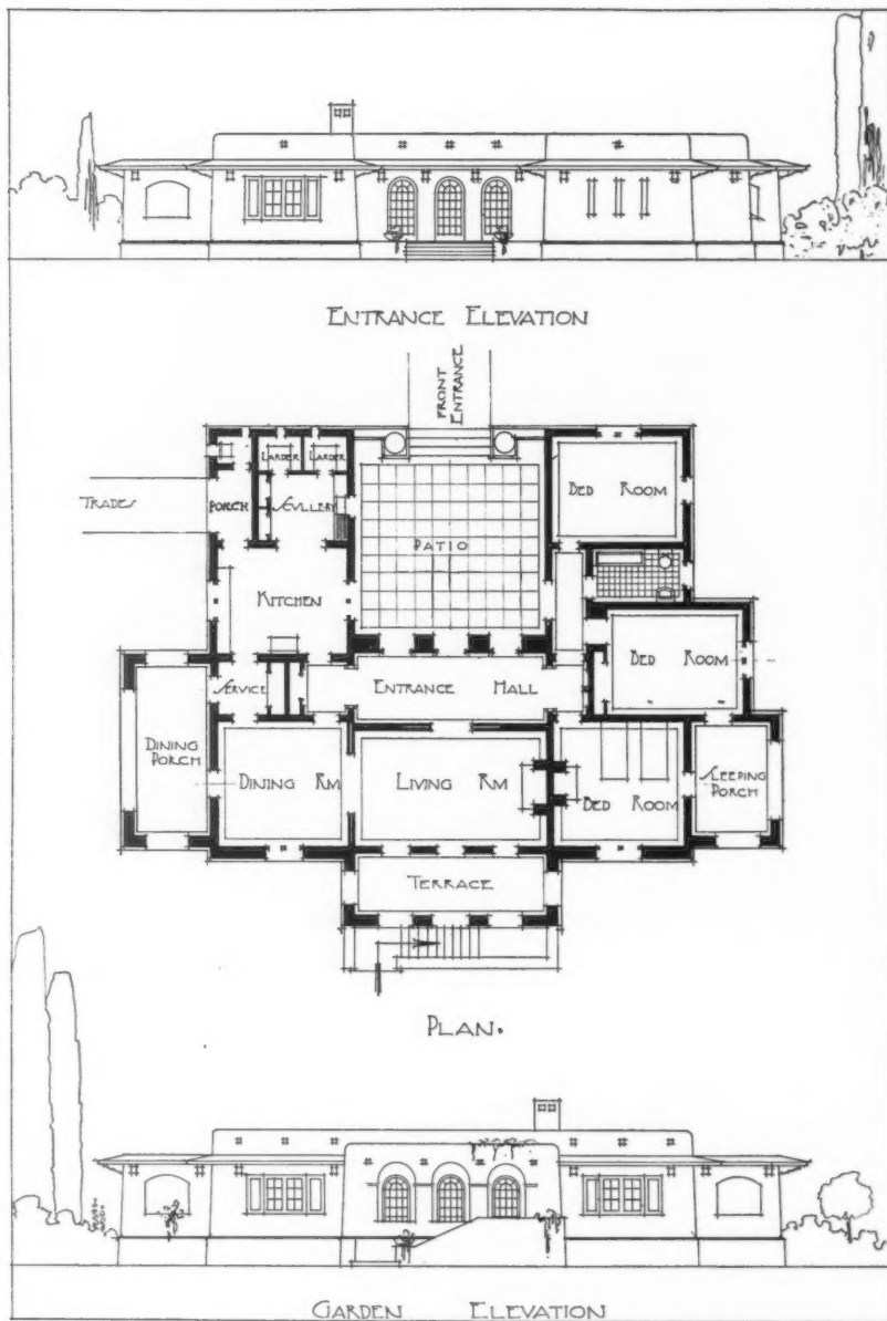
BUNGALOW IN NEW ZEALAND.
