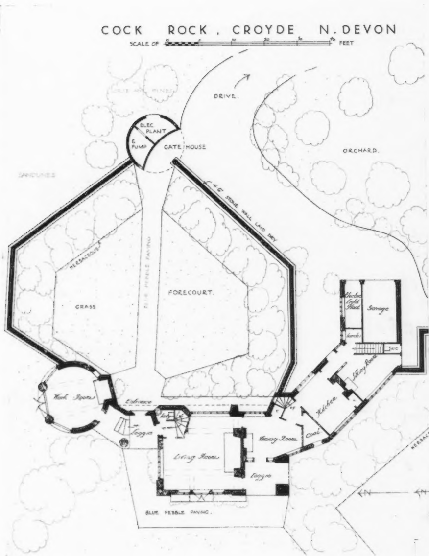
HOUSE AT CROYDE, NORTH DEVON.
