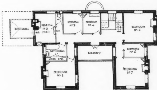
The FIRST FLOOR Plan
