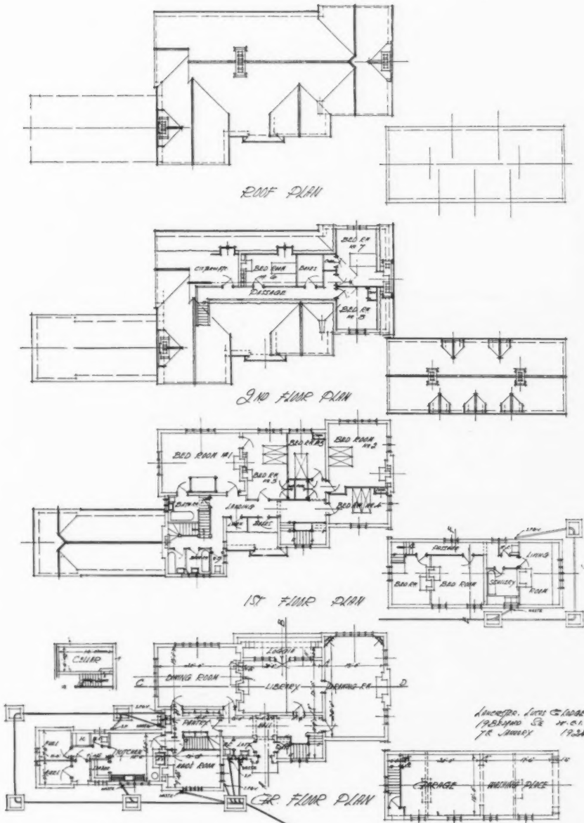
HOUSE AT OXTED.
