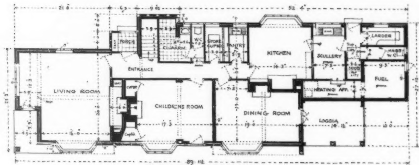
PLAN at GROUND FLOOR
