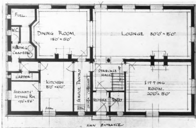
DESIGN FOR A HOUSE AT NEWBURY.
