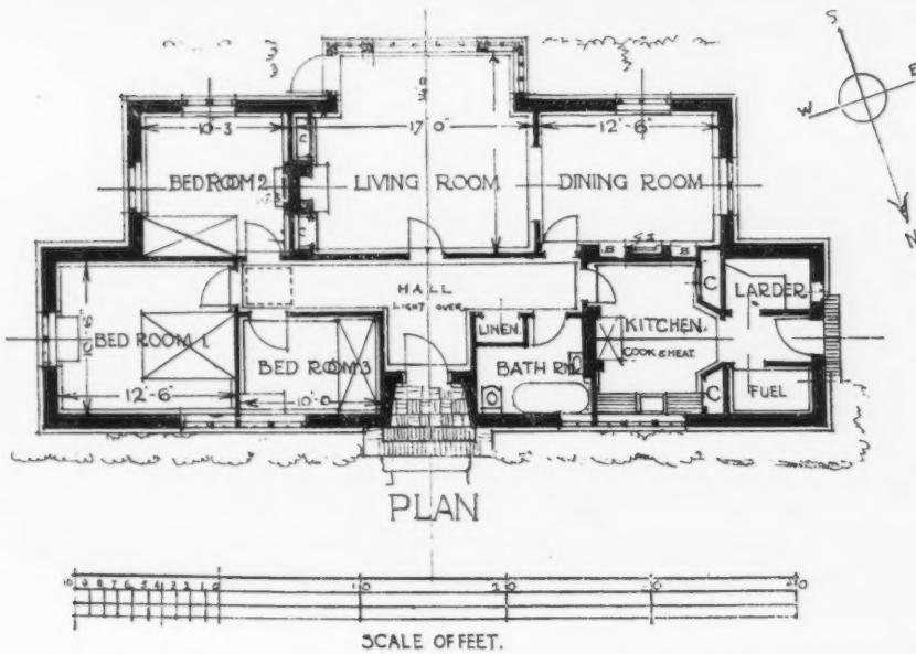
BUNGALOW AT ESHER.
