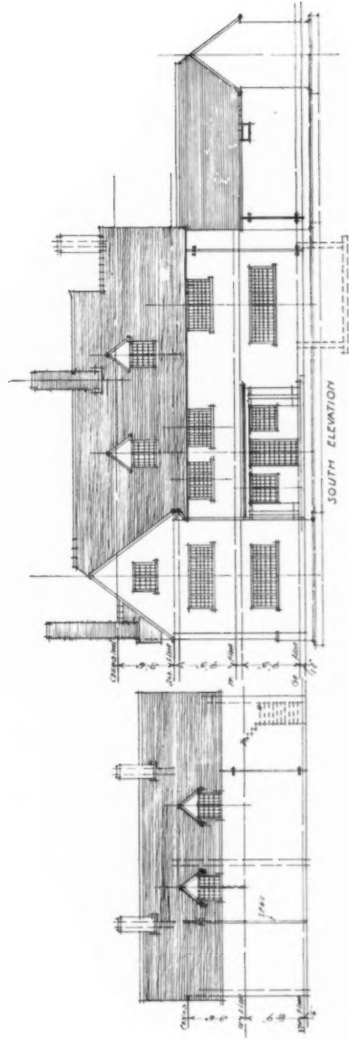
HOUSE AT OXTED : \frac{1}{8} SCALE ELEVATIONS.
