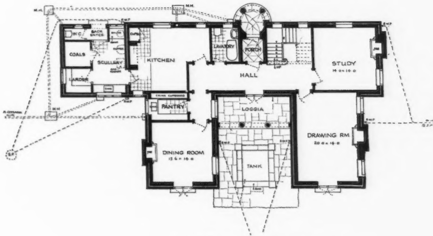
The GROUND FLOOR Plan
