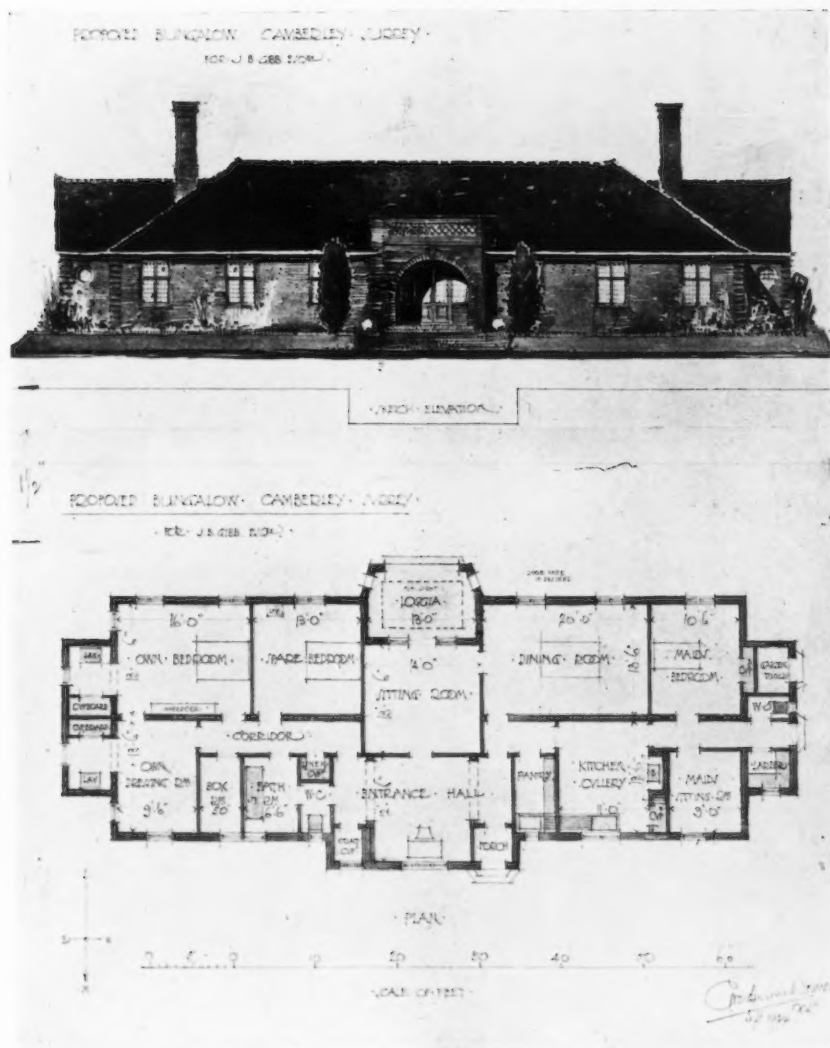
BUNGALOW AT CAMBERLEY.
