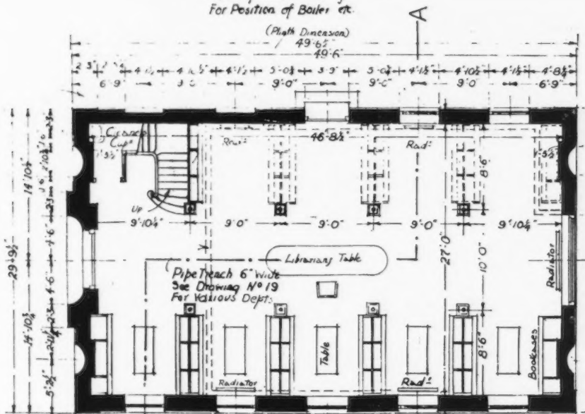
ALDENHAM SCHOOL LIBRARY.
