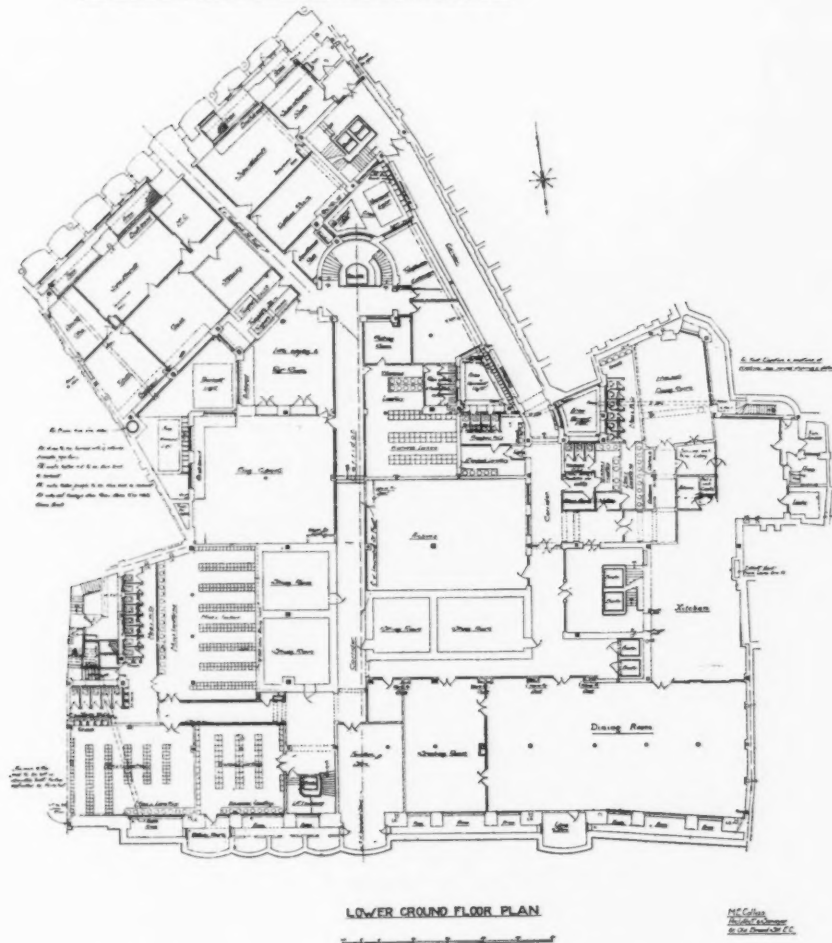
LOWER GROUND FLOOR : FURNESS HOUSE, LEADENHALL STREET, E.C.
