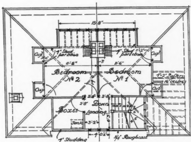
ATTIC PLAN
