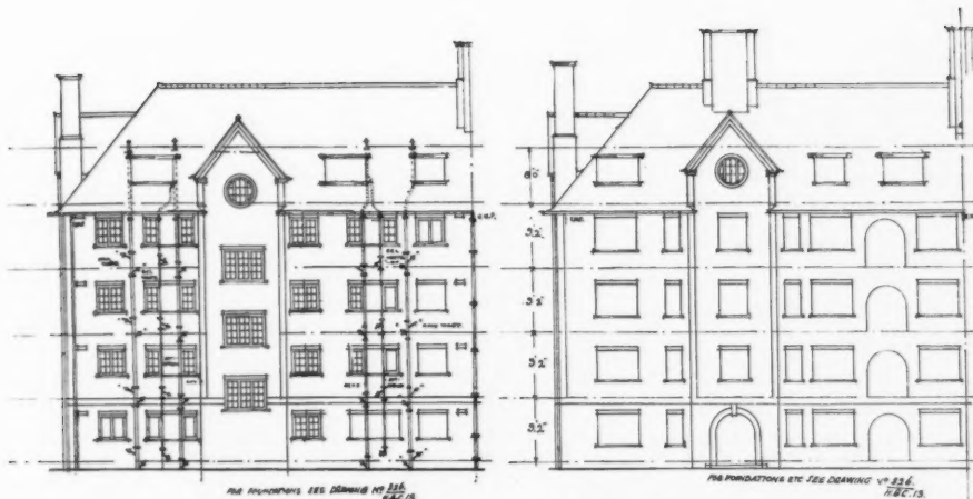
HALF NORTH ELEVATION.
