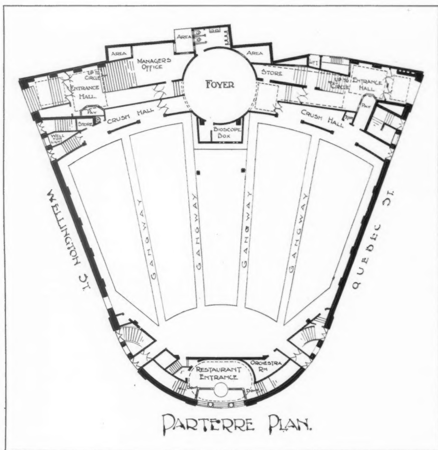
GROUND FLOOR OR PARTERRE PLAN. THE MAJESTIC PICTURE THEATRE, LEEDS. P. L. STIENLET & MAXWELL, ARCHITECTS.
