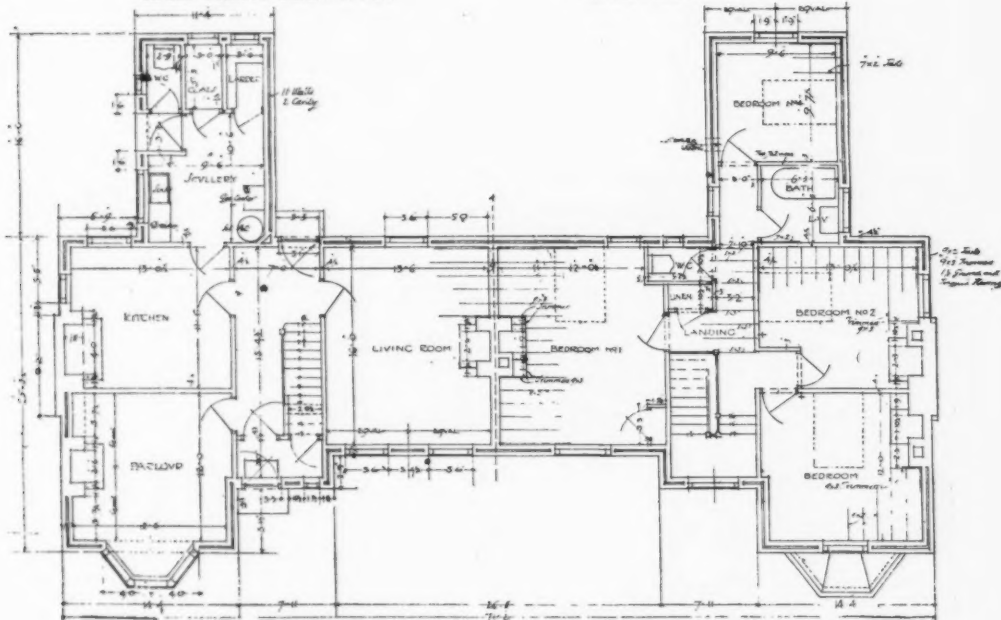
HALF-GROUND-FLOOR-PLAN
