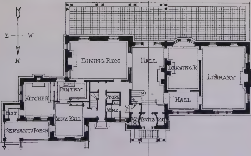
House at Ardmore, Pennsylvania, G. BISPHAM PAGE, Architect.
