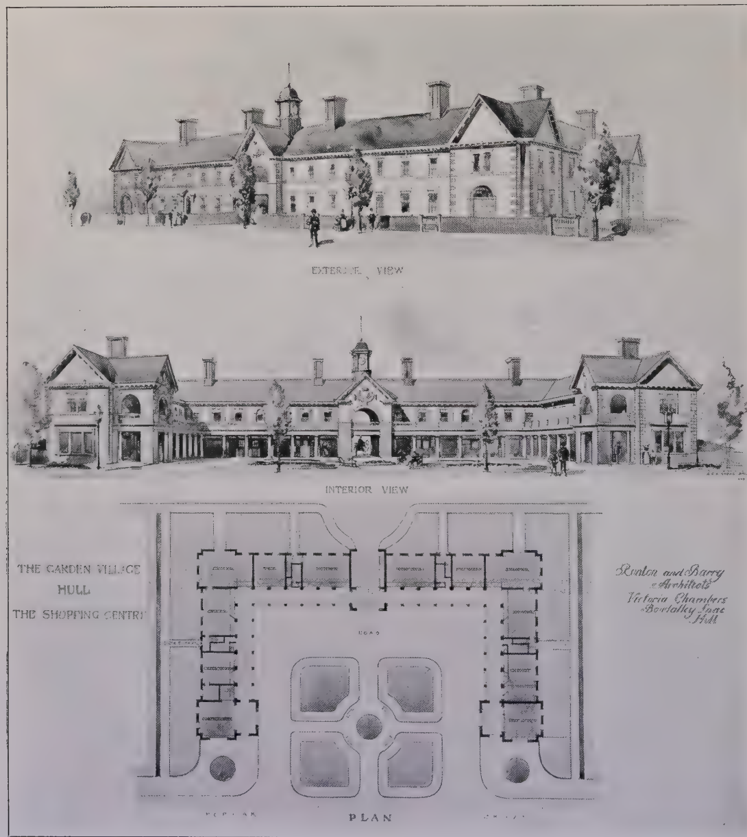
The Shopping Centre, Garden Village, Hull, RUNTUN AND BARRY, Architects.
