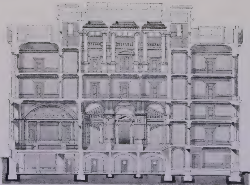
Government Buildings, Sofia, ALEX. KOCH, Architect. (For Plans, see p. 131.)
