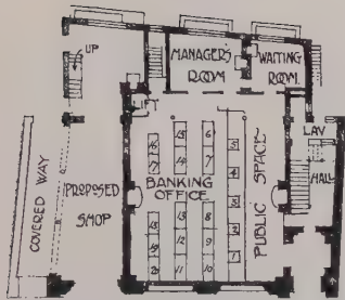
GROUND FL. PLAN.
