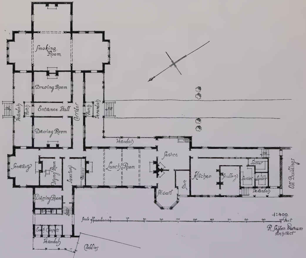
Golf Club House, Sandwich, R. SELDEN WORNUM, Architect.
