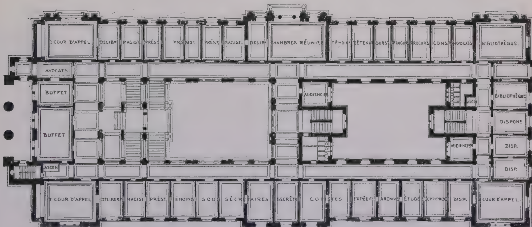
Government Buildings, Sofia, ALEX. KOCH, Architect.
