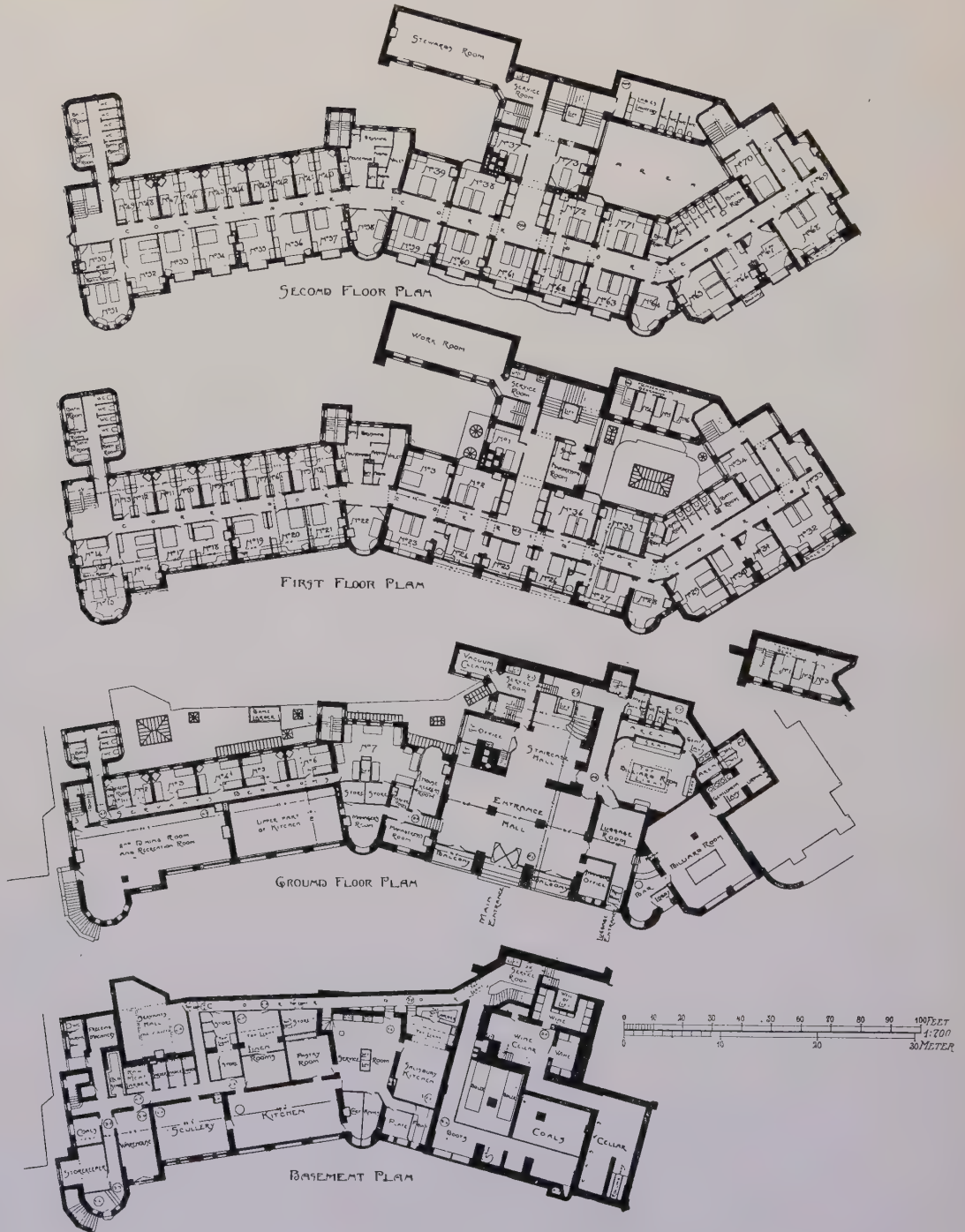
Orielton Hall, Barmouth, J. COATES CARTER, Architect.
