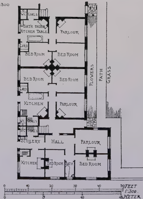
Cottage Flats, Surrey, WILLIAM HUNT, Architect.
