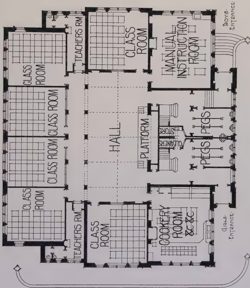
Public School, Armadale, J. GRAHAM FAIRLEY, Architect.
