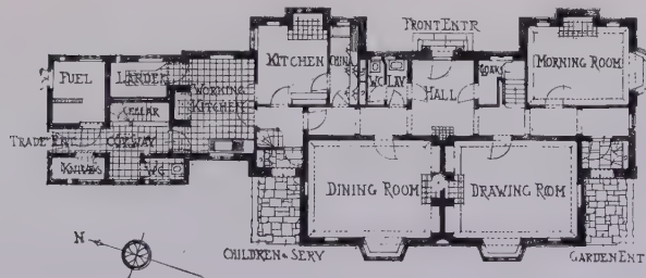
House at Darenth, Kent, WILFRID HOYLE, Architect.
