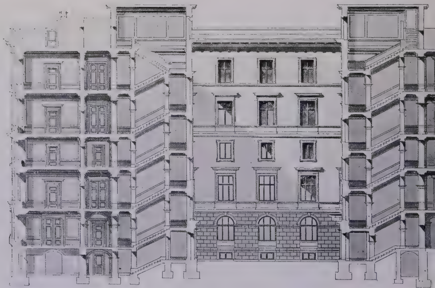
Competition Design for Governor's Office (1)
