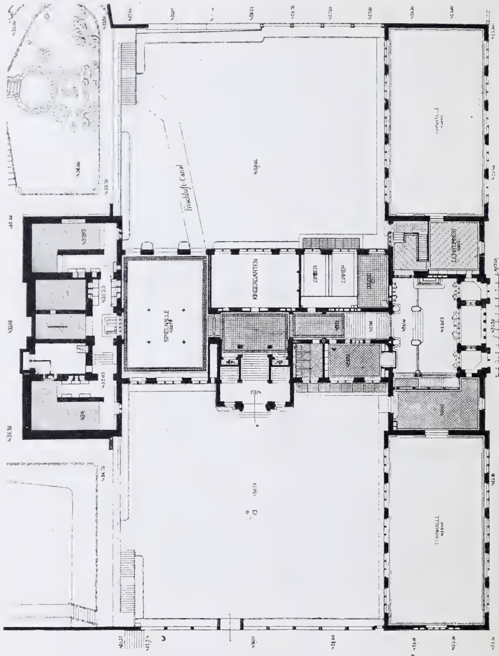
Plans, New Board School, Zürich, Switzerland , ALEX. KOCH, Architect, London. (For Elevation, see p. 123.)
