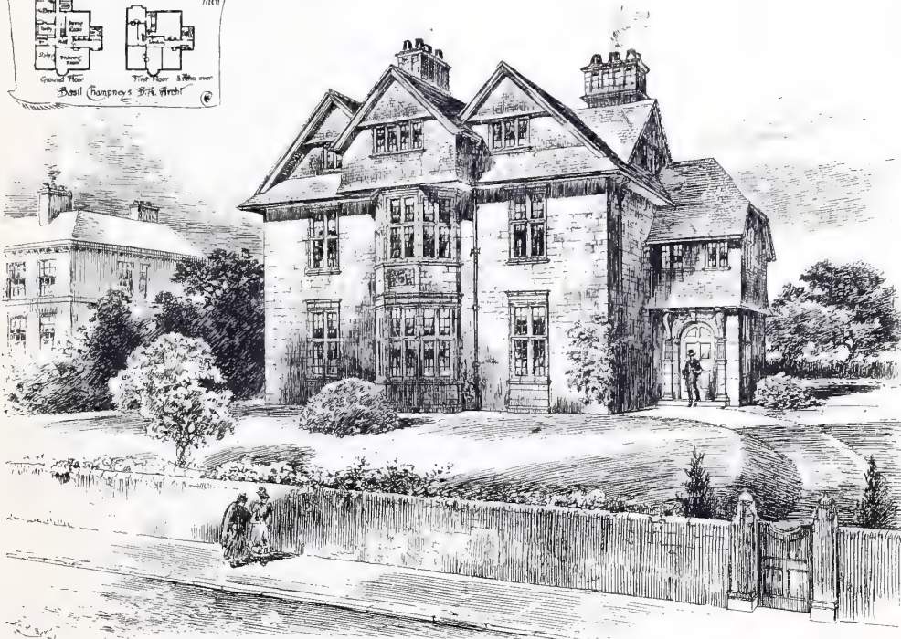
1579. Haslingden Vicarage, Lancashire , BASIL CHAMPNEYS, B.A., Architect.
