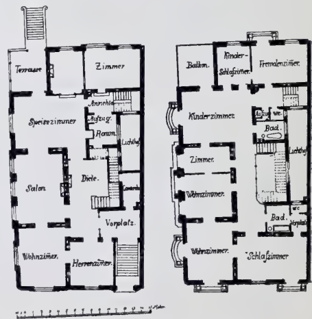
Villa Haniel, plans.
