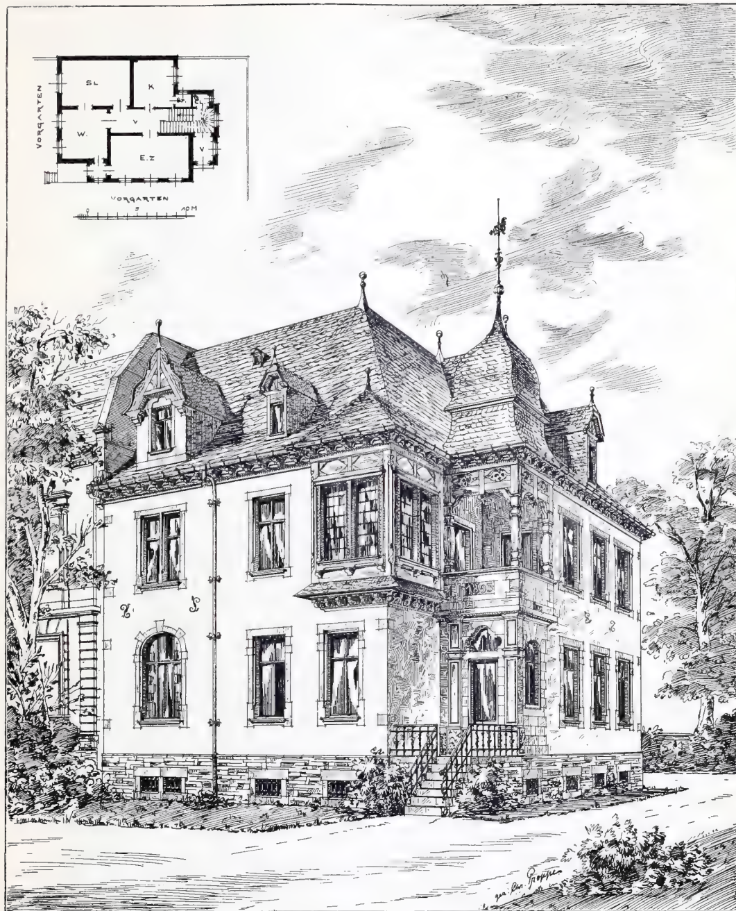
Villa Gorny, Frankfurt, H. TH. SCHMIDT, Architect, Frankfurt a/M.
