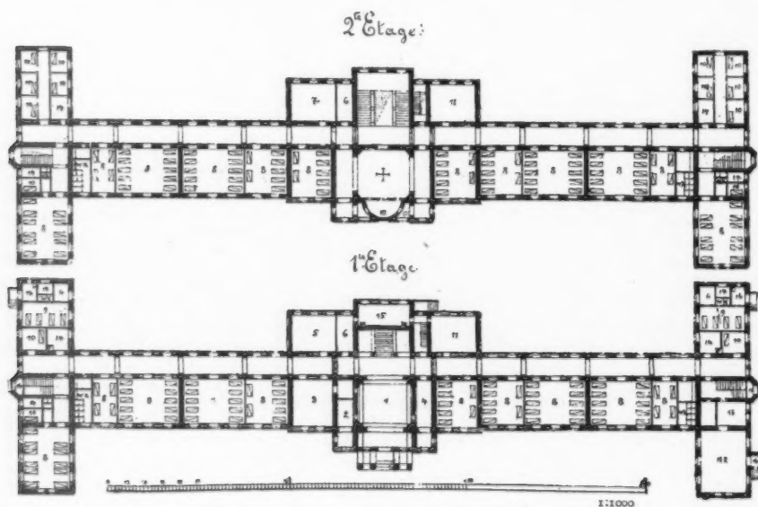
Bachruschin Bros. Hospital for Chronic Diseases, Moscow, B. FREUDENBERG, Architect, Moscow.
