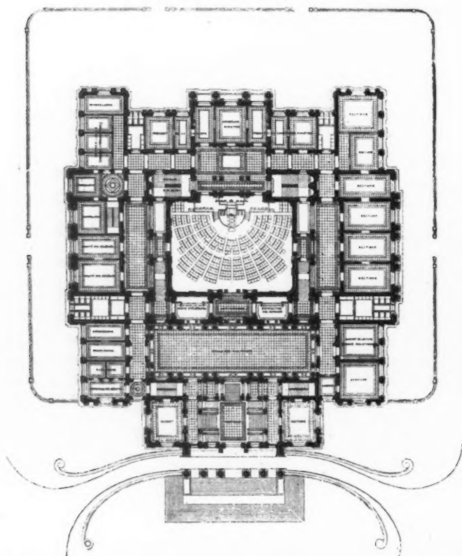
1901. Competition Design for "Le Palais de la Chambre des Députés," Bukarest (mention honorable), ALEX. KOCH, Architect
