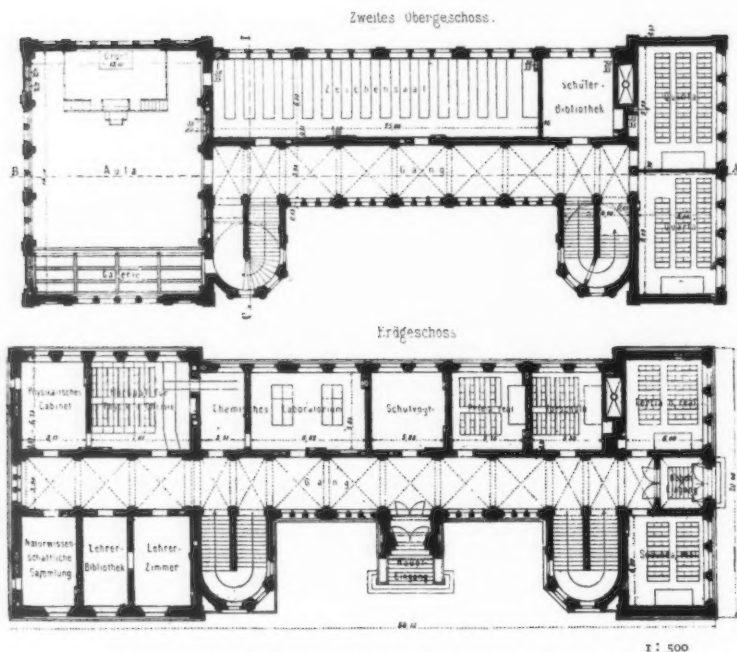
Gymnasium and Real Gymnasium (Classical School) Goslar, Germany. PROF. HUBERT STIER, Architect, Hanover. Elevation, p. 96.
