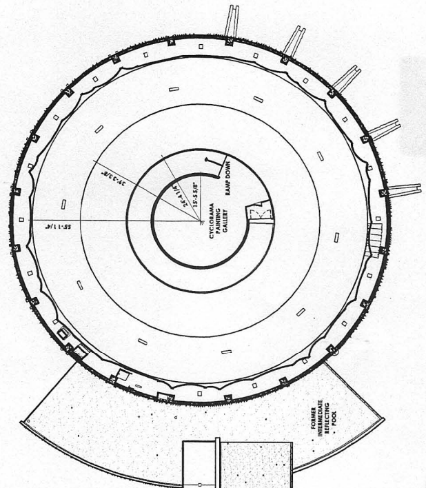
ROOF PLAN 3/32"=1'-0" 1:126
