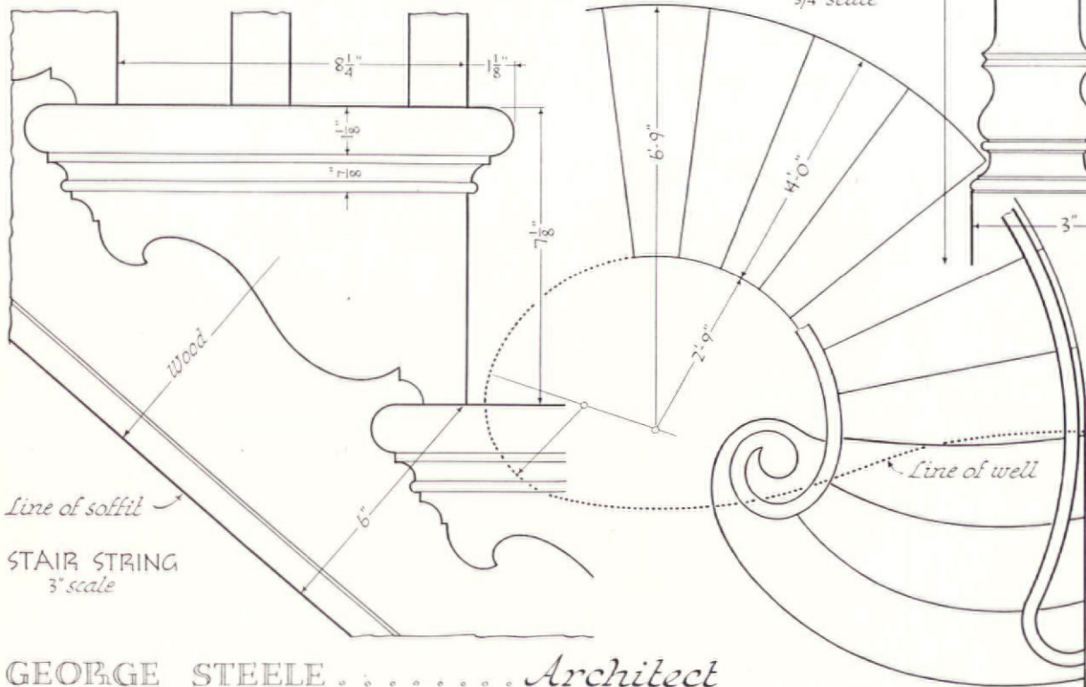
PLAN of STAIRS 3/4" scale
