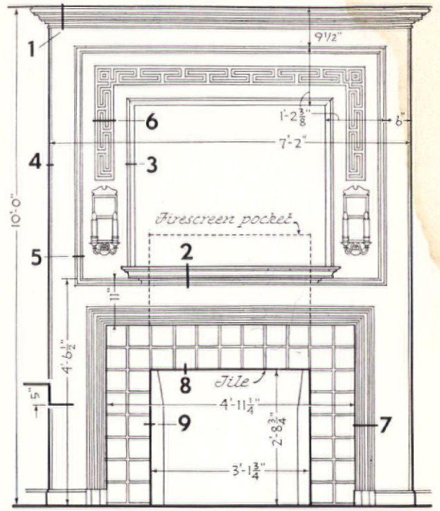
ELEVATION 3/8" scale
