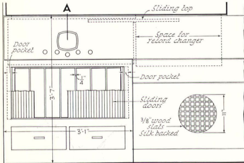
ELEVATION 3/4" scale
