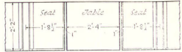
PLAN of SEATS 3/8" scale
