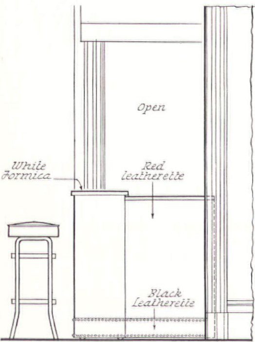
SIDE ELEVATION 1/2" scale
