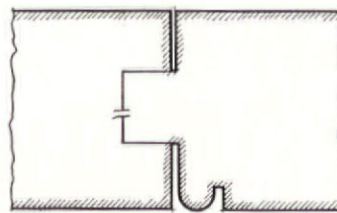
SECTION 1 Full size
