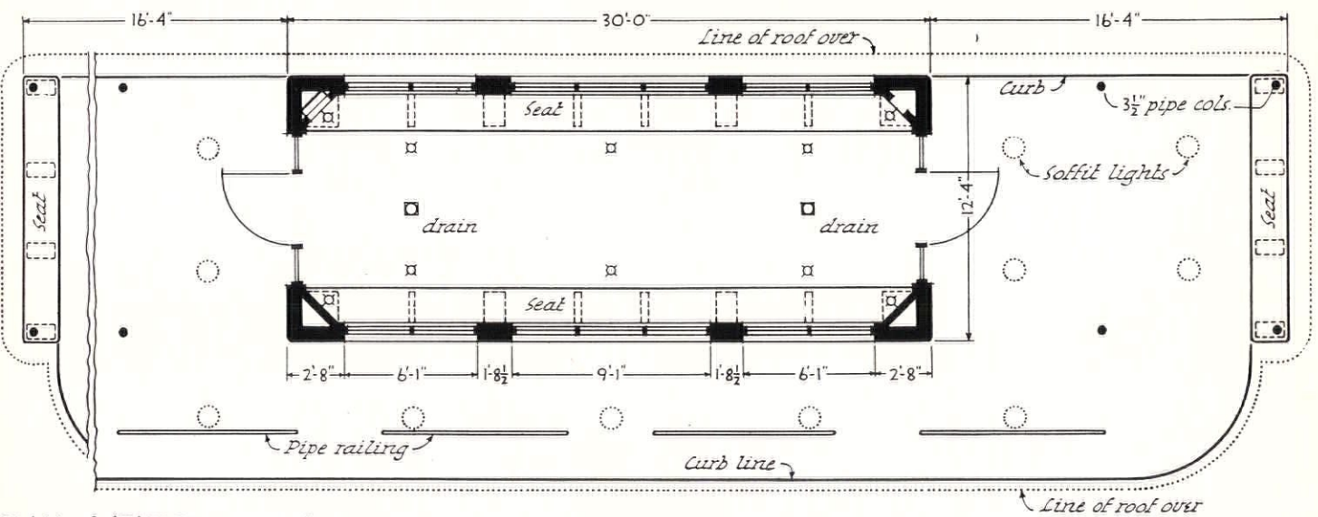
PLAN of STATION 1/8" scale
