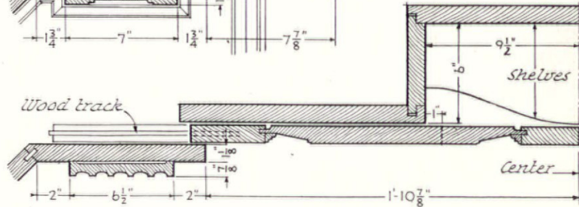
SECTION A 1\frac{1}{2} " scale
