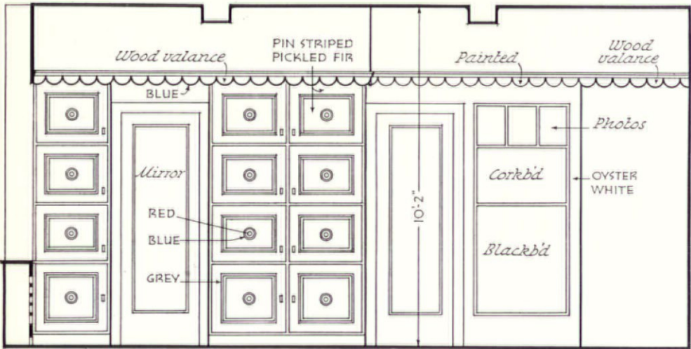
ELEVATION towards 3
