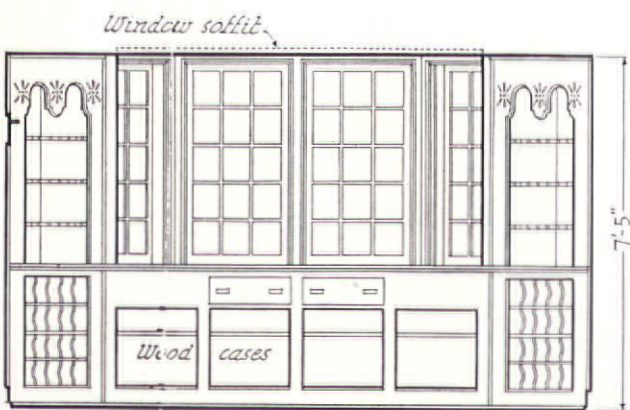
ELEVATION 1/4" scale
