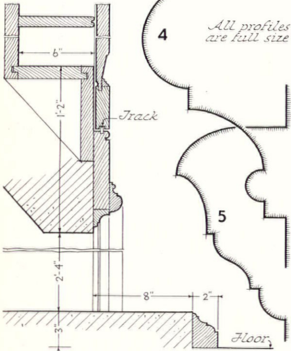
SECTION C
