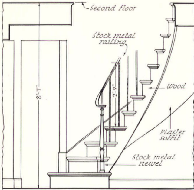
ELEVATION \frac{3}{8} " scale
