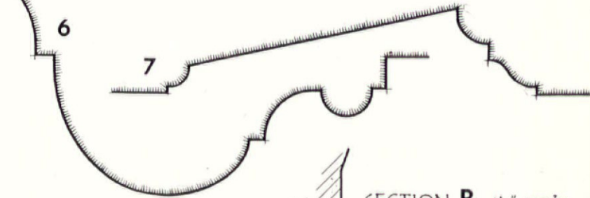
SECTION B 1\frac{1}{2} " scale
