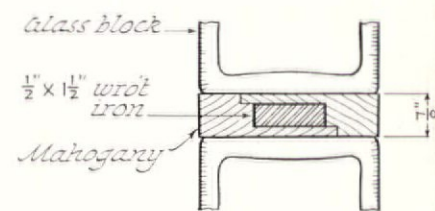
SECTION 3
