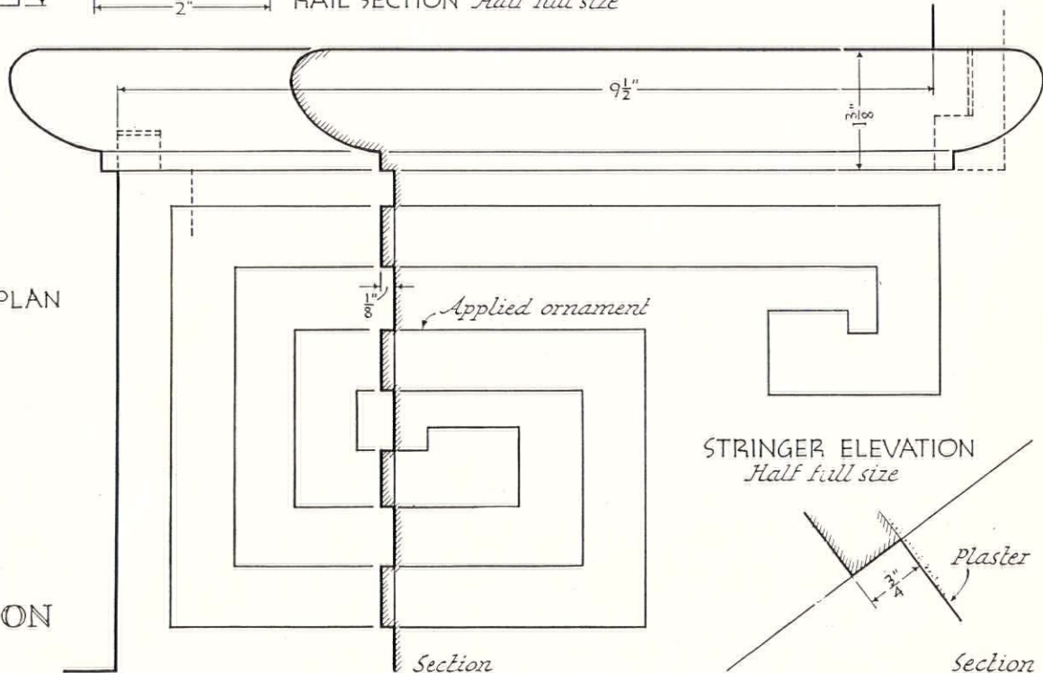
RAIL SECTION Half full size
