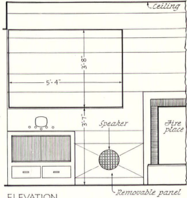
ELEVATION 3/8" scale
