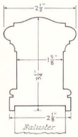
HANDRAIL Half full size
