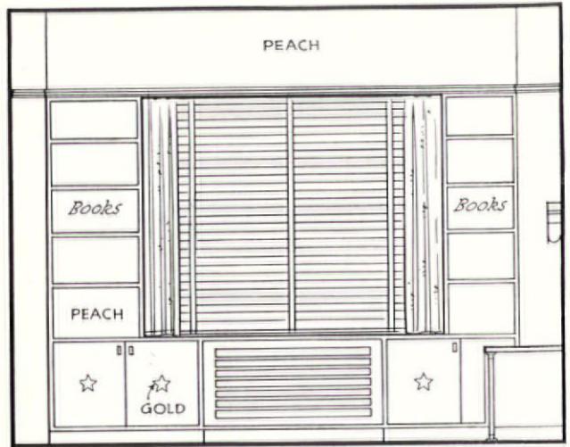
ELEVATION towards 3
