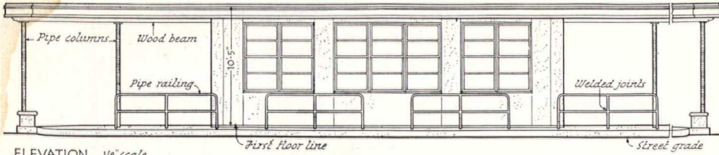
ELEVATION 1/8" scale
