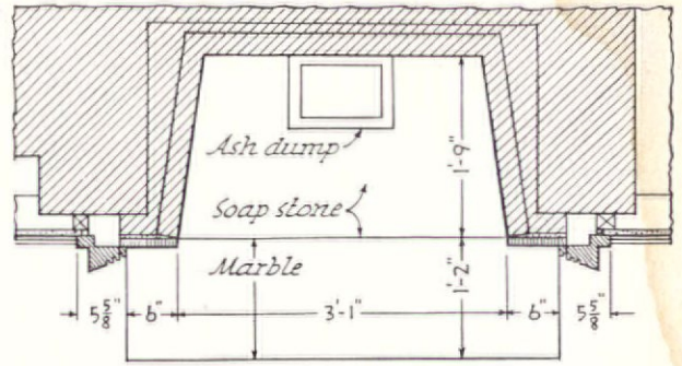
PLAN 1/2" scale
