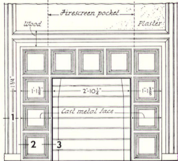
ELEVATION 1/2" scale
