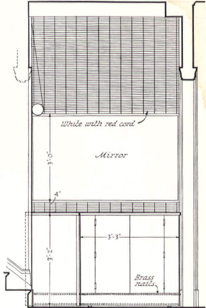
FRONT ELEVATION 1/2" scale
