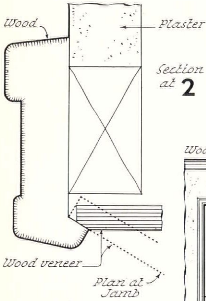
SECTIONS at FULL SIZE
