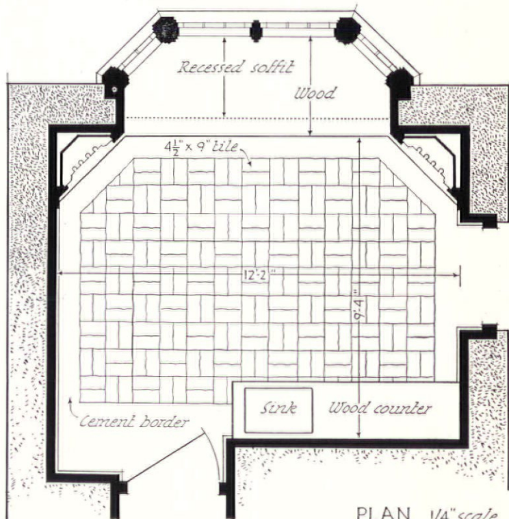
PLAN 1/4" scale
