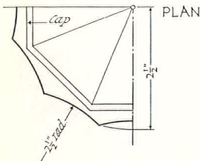
NEWEL POST Half full size
