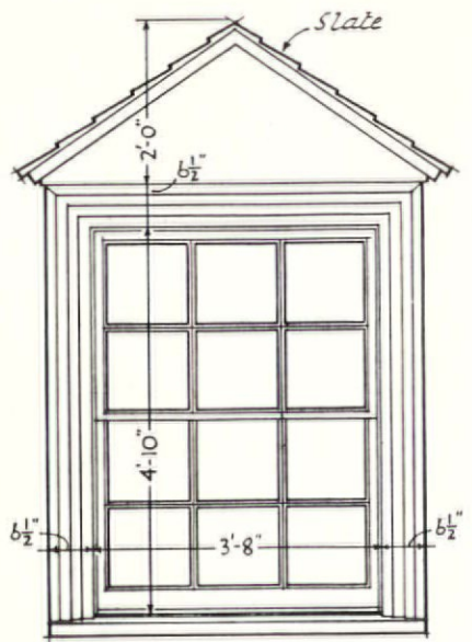
DORMER ELEVATION 3/8" scale
