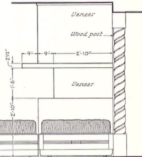
ELEVATION 3/8" scale
