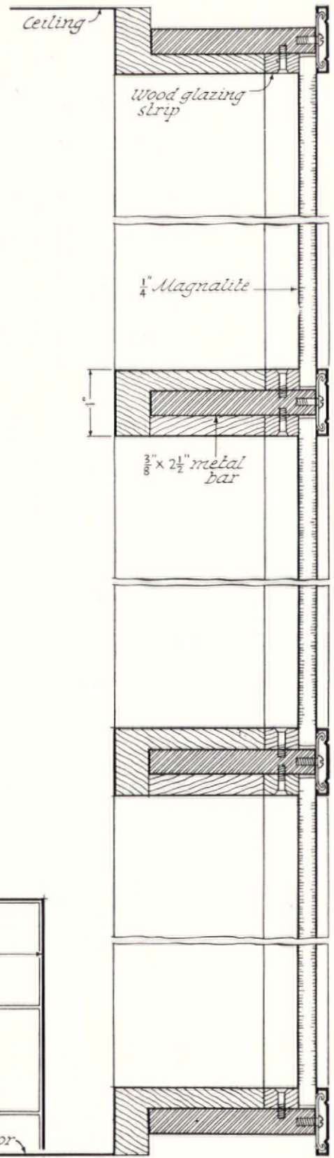
WINDOW SECTION Half full size
