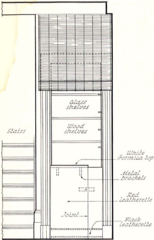
ELEVATION \frac{1}{2} " scale
