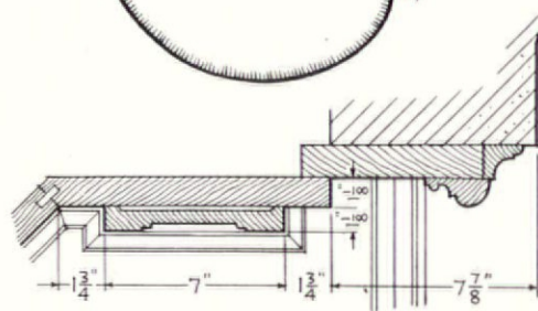
SECTION B 1\frac{1}{2} " scale
