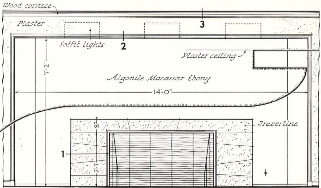
ELEVATION 3/8" scale
