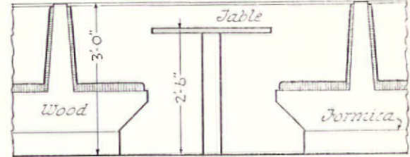
ELEVATION of SEATS
