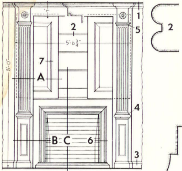
ELEVATION \frac{3}{8} " scale
