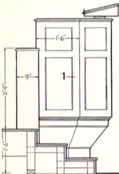
SIDE ELEVATION \frac{1}{2} " scale
