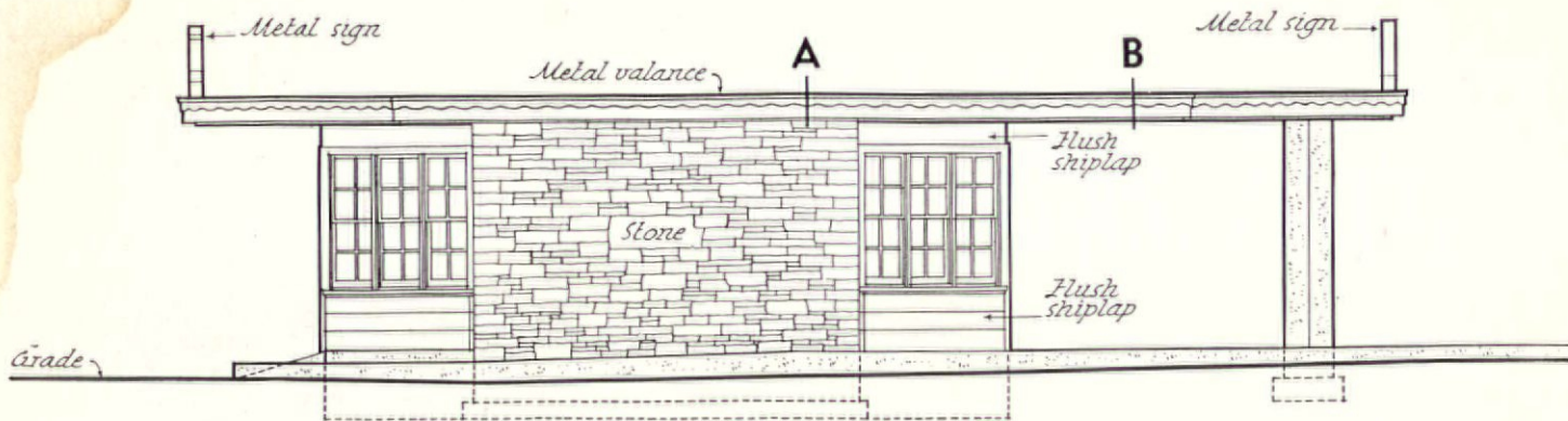
SIDE ELEVATION
