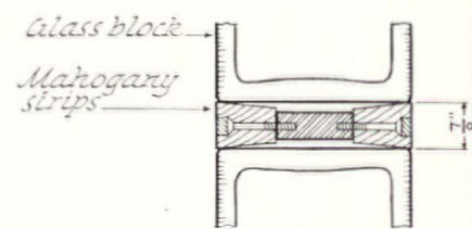
SECTION 4
