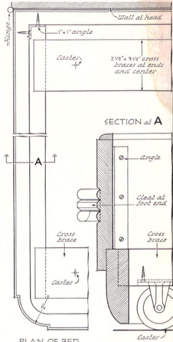
PLAN OF BED 3" scale
