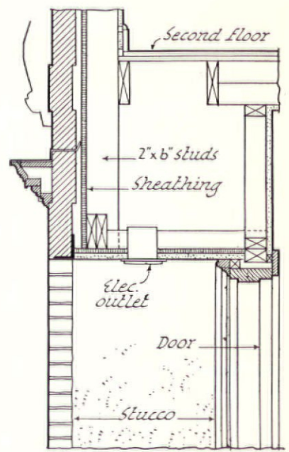
SECTION thru HEAD 1/2" scale
