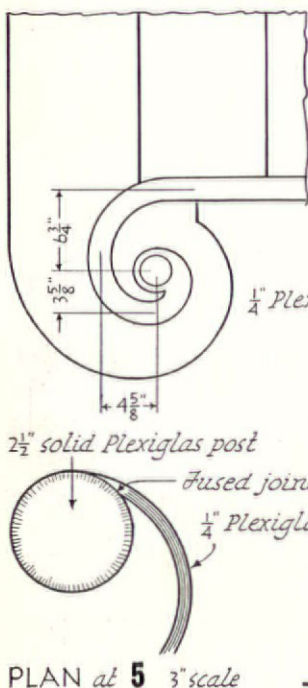
PLAN AT NEWEL 3/4" scale
