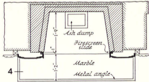
PLAN 1/2" scale
