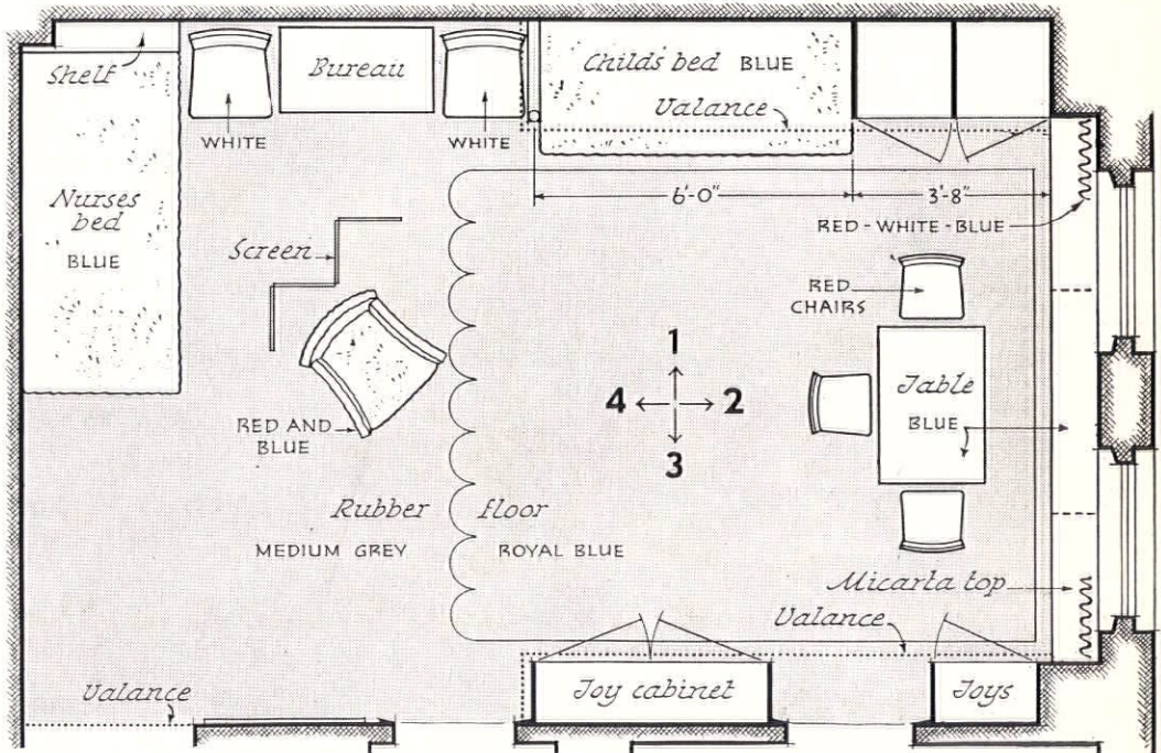
PLAN 1/4" scale
