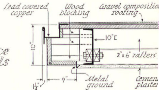
SECTION B 3/4" scale
