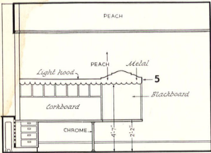
ELEVATION towards 4 1/4" scale
