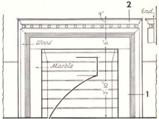
ELEVATION 1/2" scale
