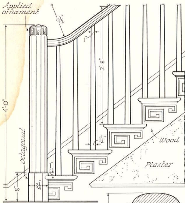
ELEVATION 3/4 " scale
