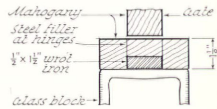
SECTION 2
