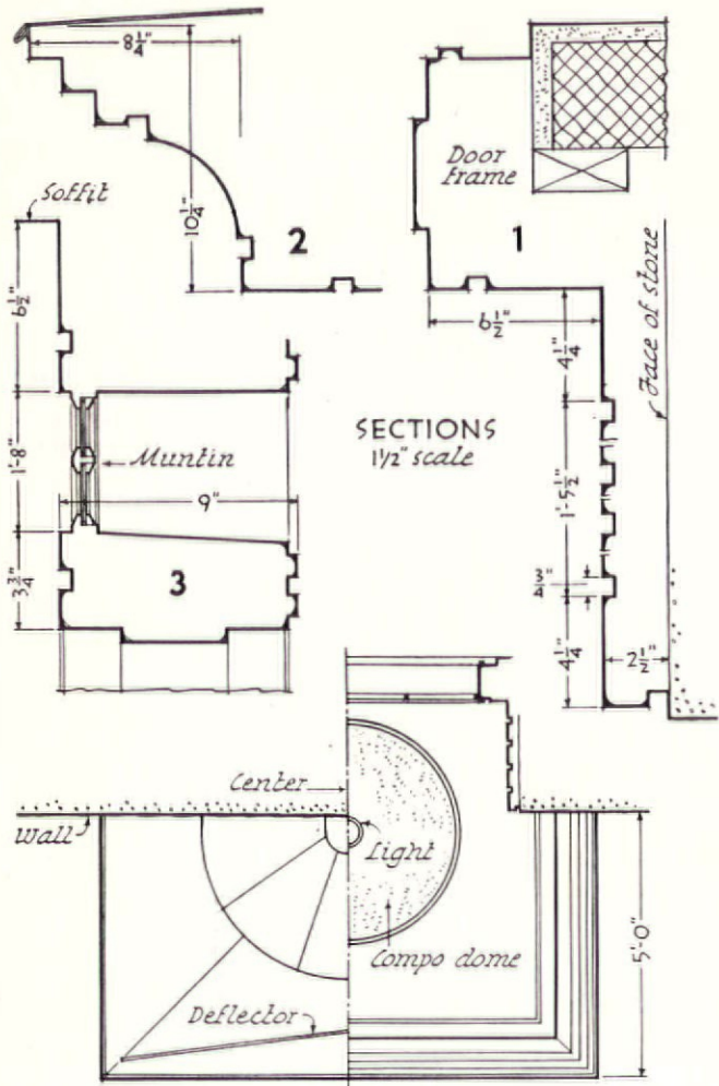
PLAN 1/4" scale
