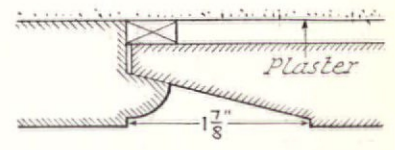
PANEL MOULD Half full size
