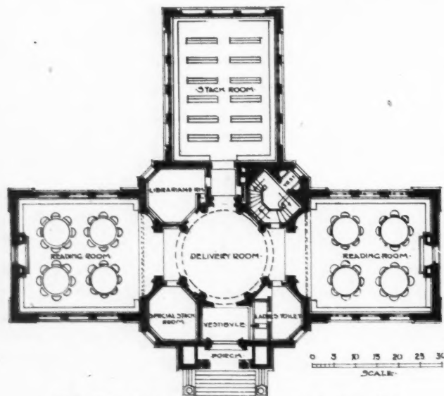
FIRST STORY PLAN, JUNIATA COLLEGE LIBRARY. (FIG. 25.)
