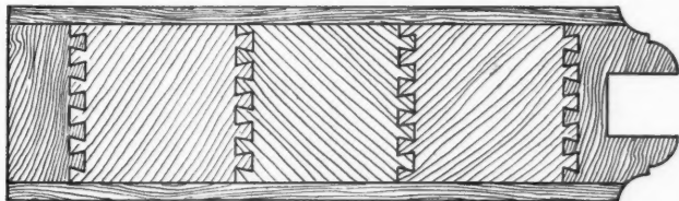
THE "KORELOCK"—A PERFECT CORE.
