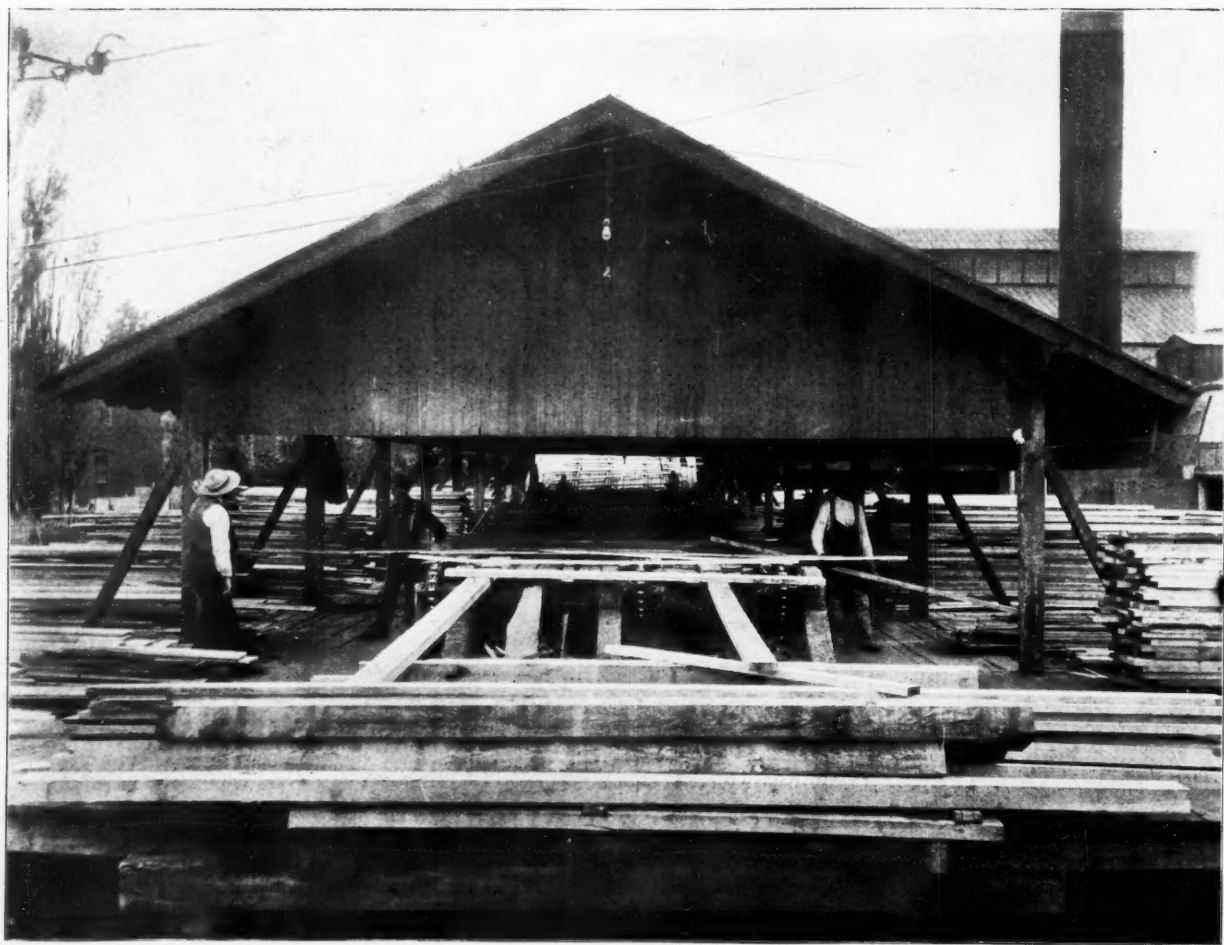
LUMBER COMING FROM SAW MILL ON SORTING CHAINS.
