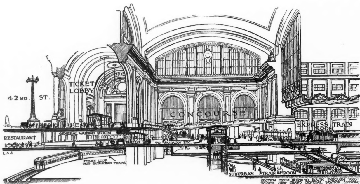
SECTION, GRAND CENTRAL TERMINAL.
