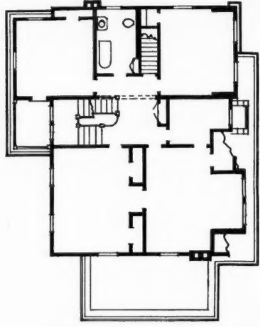
FLOOR PLANS.
