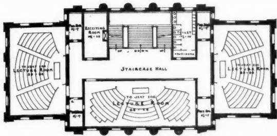
ADMINISTRATION—SECOND FLOOR.
