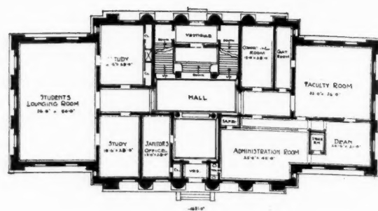
ADMINISTRATION—FIRST FLOOR.
