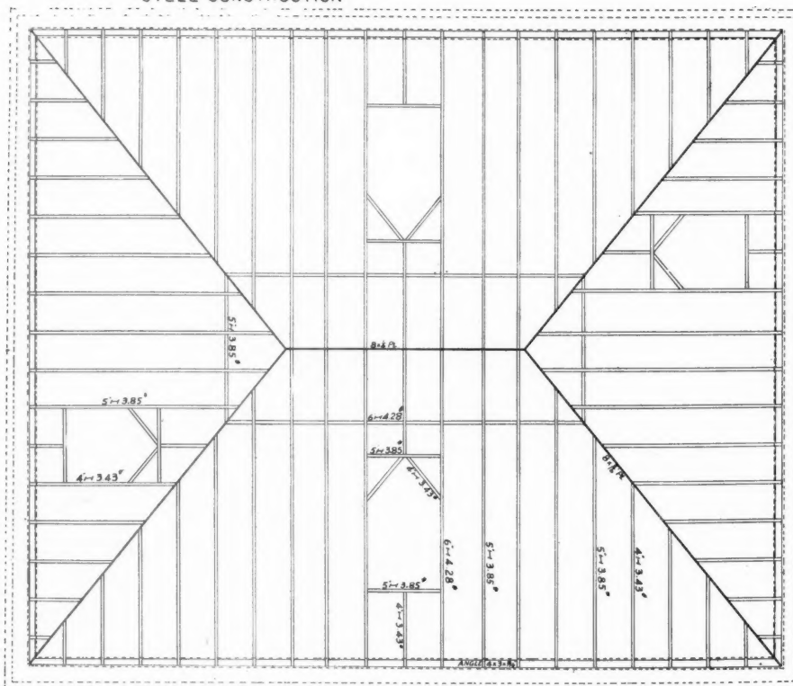
ROOF PLAN
