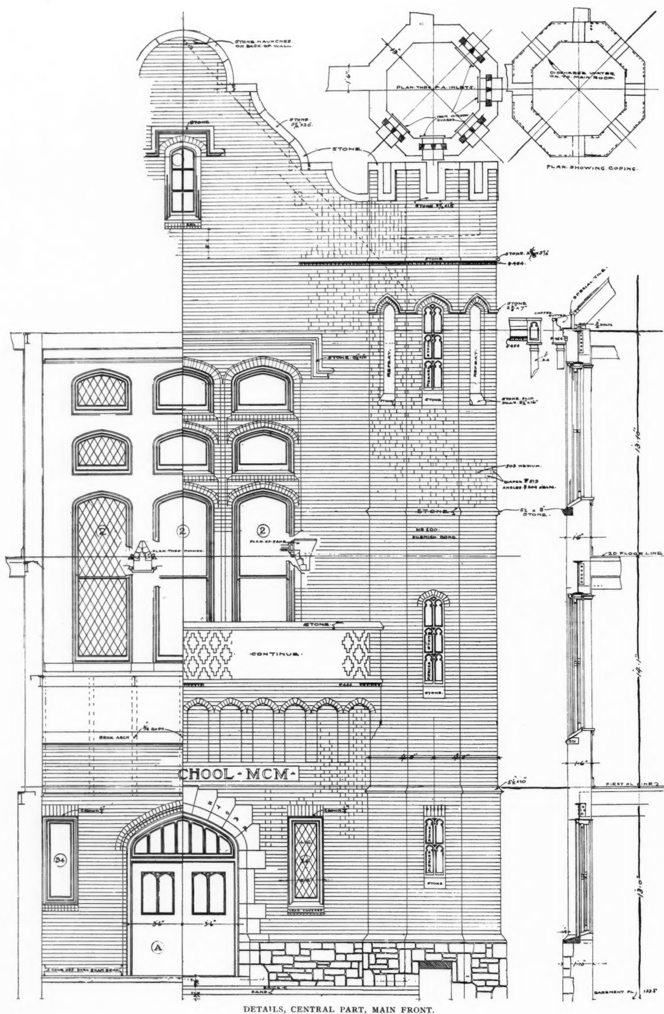
THE EDWARD WYMAN SCHOOL WILLIAM B. ITTNER
