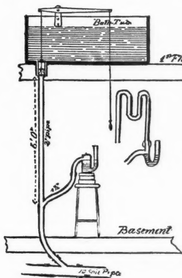
FIG. 21. SIMPLER FORM OF HYDRAULIC TESTING APPARATUS.
