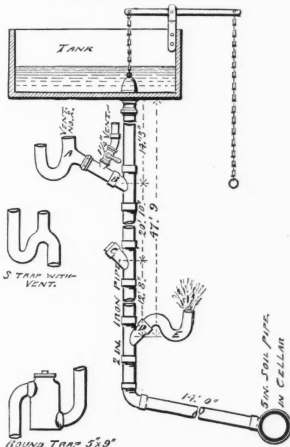
FIG. 22. APPARATUS USED AT THE "WORCESTER TESTS."
