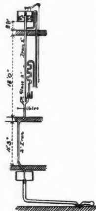
FIG. 20. APPARATUS USED AT THE NORTH END UNION.
