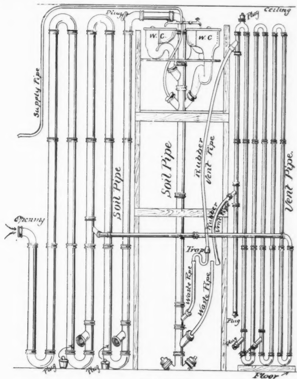
FIG. 18. APPARATUS USED AT THE MASSACHUSETTS INSTITUTE OF TECHNOLOGY.
