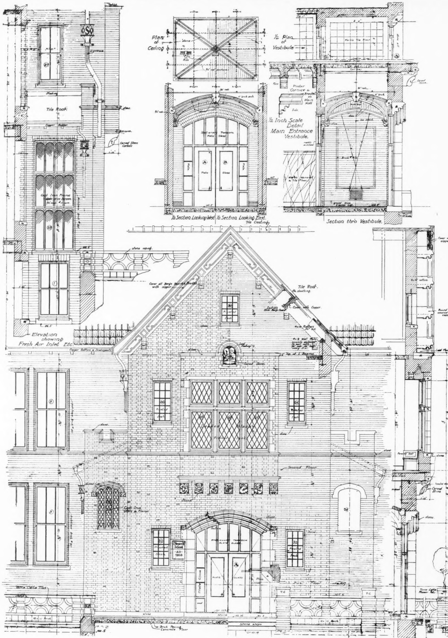
DETAILS, SHEPARD SCHOOL BUILDING, ST. LOUIS, MO.
