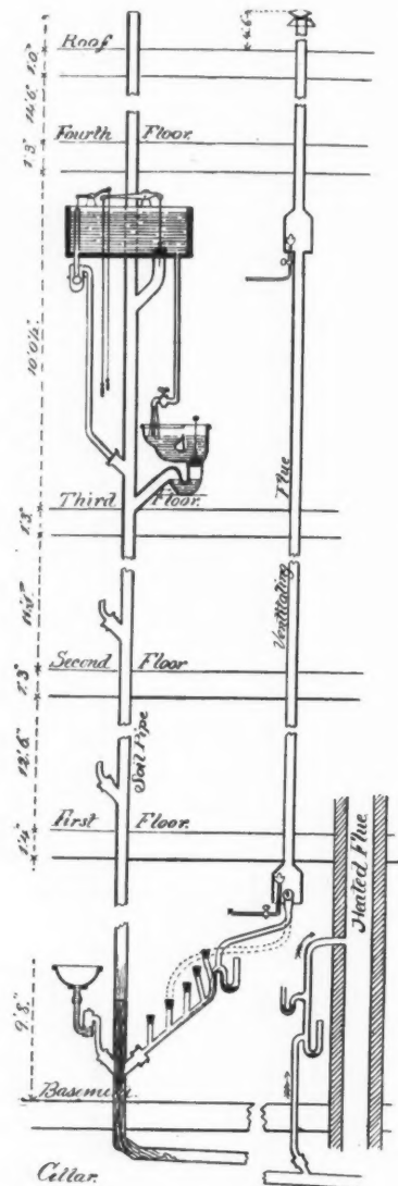
FIG. 19. APPARATUS USED IN THE EXPERIMENTS FOR THE BOSTON CITY BOARD OF HEALTH.
