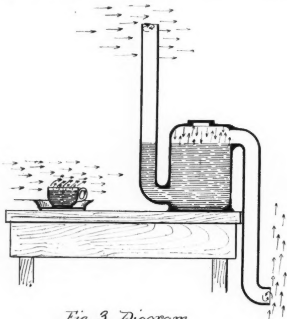
Fig. 3. Diagram illustrating the Air Movements above the Water Seal of a Back Vented S Trap, and of a Non Vented Antisiphon Trap. The Former quickly losing, and the Latter indefinitely retaining its Seal.
