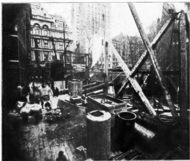
THE TRINITY CAISSON FOUNDATIONS. THE FOUNDATION COMPANY, NEW YORK.
