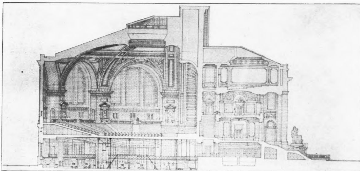
TRANSVERSE SECTION
