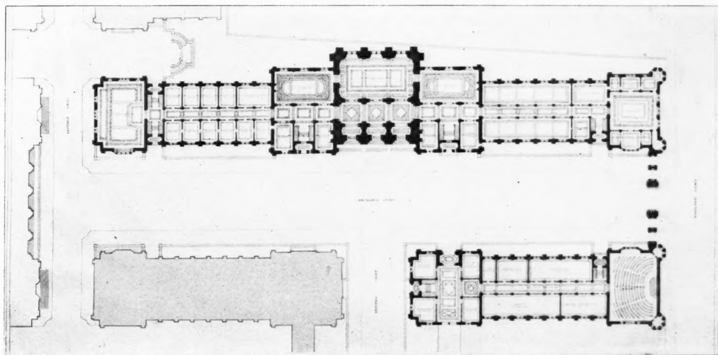
ADMINISTRATION GROUP. PLAN OF MAIN BUILDING, Applied Science Group, Div. A, First Floor Plan
