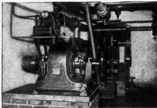
Westinghouse Type M Direct Current Motor Driving Pump
