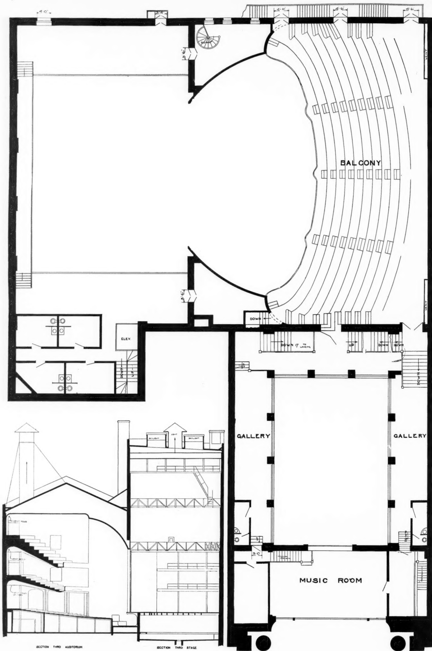
BALCONY FLOOR PLAN
