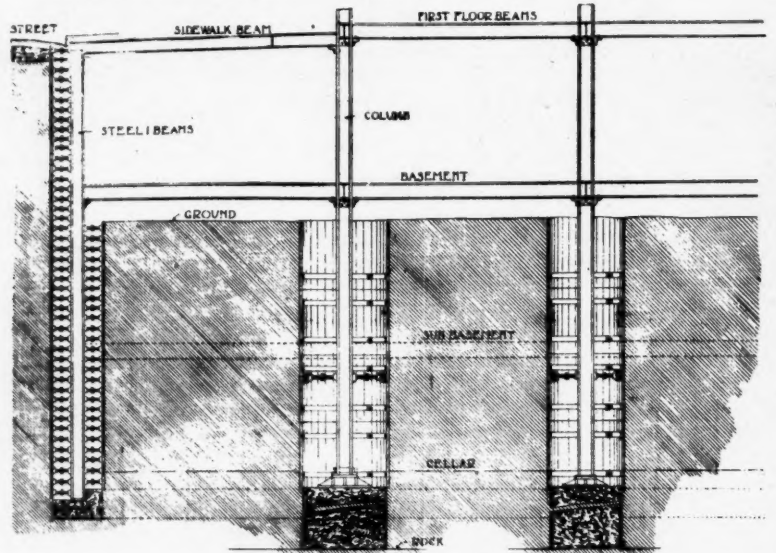
GENERAL SECTION SHOWING EXCAVATION PARTIALLY MADE.
