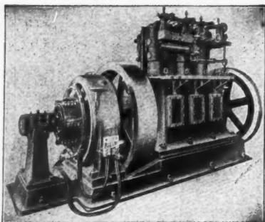
Westinghouse Gas Engine Generating Set.
