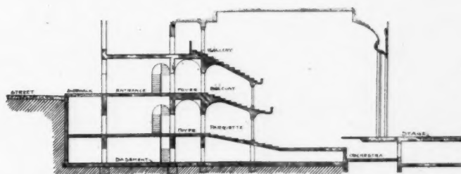
THEATER BALCONY ON LEVEL WITH THE SIDEWALK.
