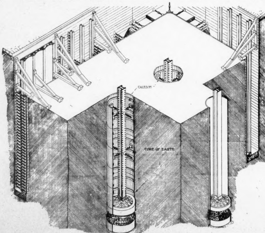
NO. 2. CAISSONS SUNK, COLUMNS IN PLACE, READY FOR SUPERSTRUCTURE.
