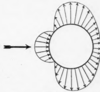
FIG. 6. Diagram illustrating wind pressure on a cylindrical body
