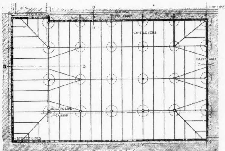
FRAMING PLAN OF BASEMENT AT A A.
