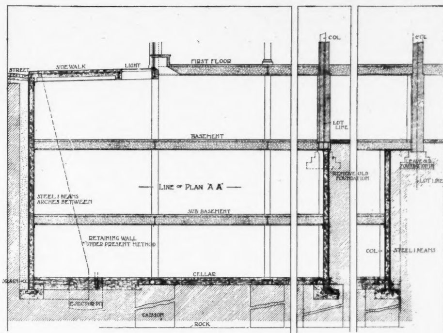
NO. 4. SECTION OF RETAINING WALL.
