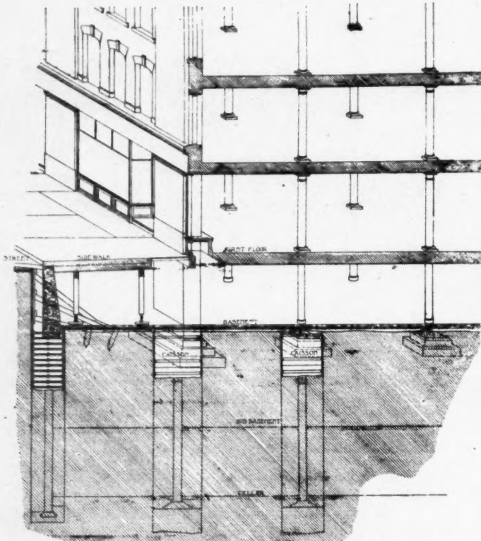
NO. 1. GENERAL SECTION, SHOWING METHOD OF BUILDING RETAINING WALLS. PATENTED JANUARY 13, 1903.
