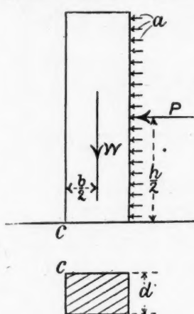
FIG. 7. Diagram illustrating the stability of a column.
