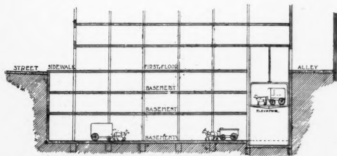
DELIVERY WAGONS LOADING IN BASEMENT INSTEAD OF ON STREET.
