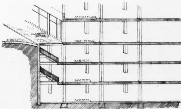
OPEN GALLERIES IN SUB-BASEMENTS FOR STORES WITH GLASS SIDEWALK.
