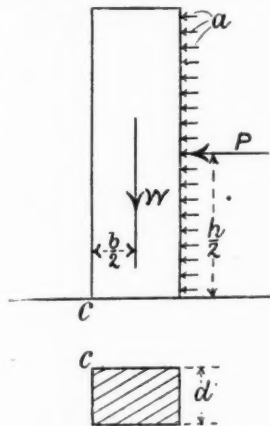
FIG. 7. Diagram illustrating the stability of a column.
