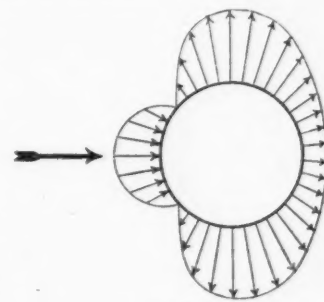
FIG. 6. Diagram illustrating wind pressure on a cylindrical body
