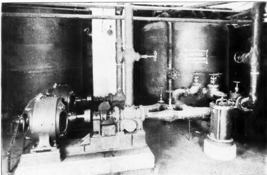
WATER FILTER AND SCREW PUMPS, PURE WATER SUPPLY.
