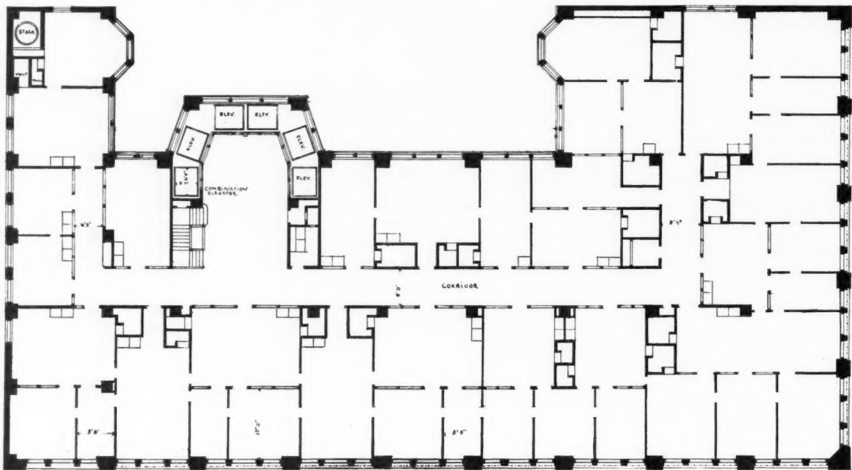
TYPICAL OFFICE FLOOR PLAN.
