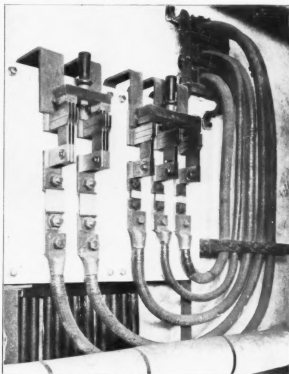
ELECTRICAL POWER CONDUCTORS, FROM THE CHICAGO EDISON CO.
