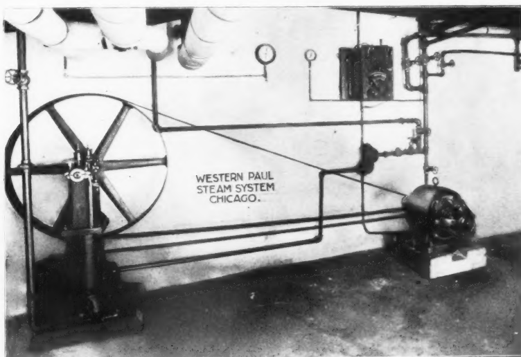
VIEW OF EXHAUSTER AND MOTOR OF PAUL SYSTEM, IN HEATING SYSTEM.
