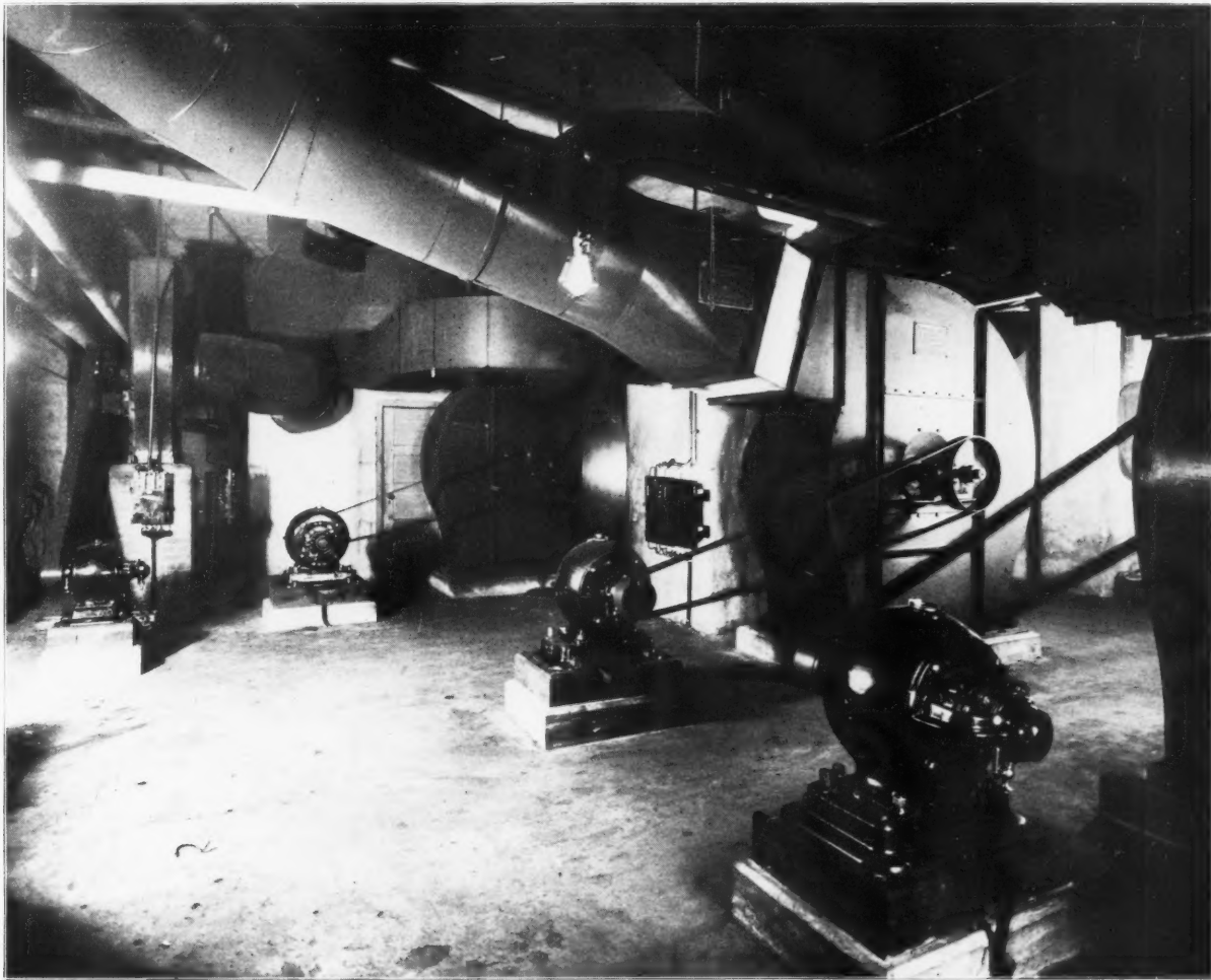
GENERAL VIEW OF VENTILATING SYSTEM, SHOWING BATTERY OF ELECTRICAL MOTORS, BLOWERS AND EXHAUSTERS.
