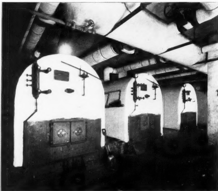
VIEW OF BATTERY OF BOILERS FOR HEATING SYSTEM.
