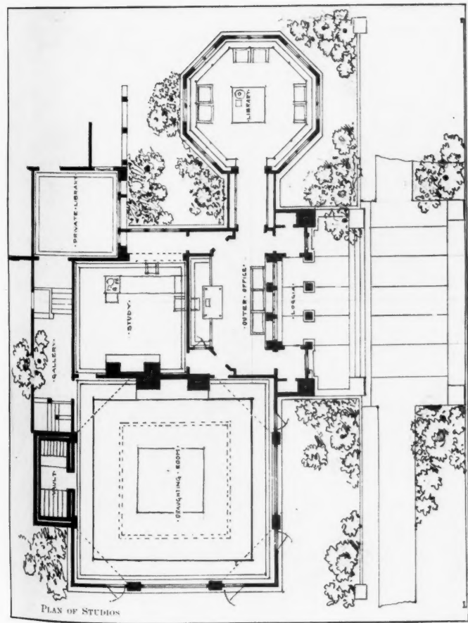
PLAN OF STUDIO.
