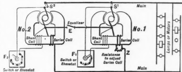
FIG. 4.—COMPOUND-WOUND DYNAMOS IN PARALLEL.
