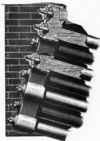
FIG. 2.—WATER-TUBE TYPE OF BOILER.
