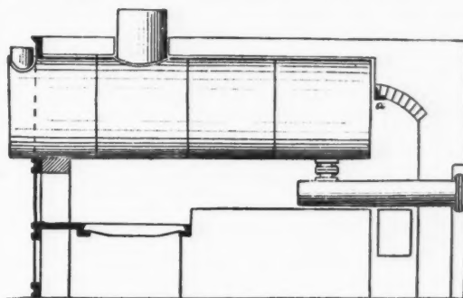
FIG. 1.—THE FIRE-TUBE TYPE OF BOILER.
