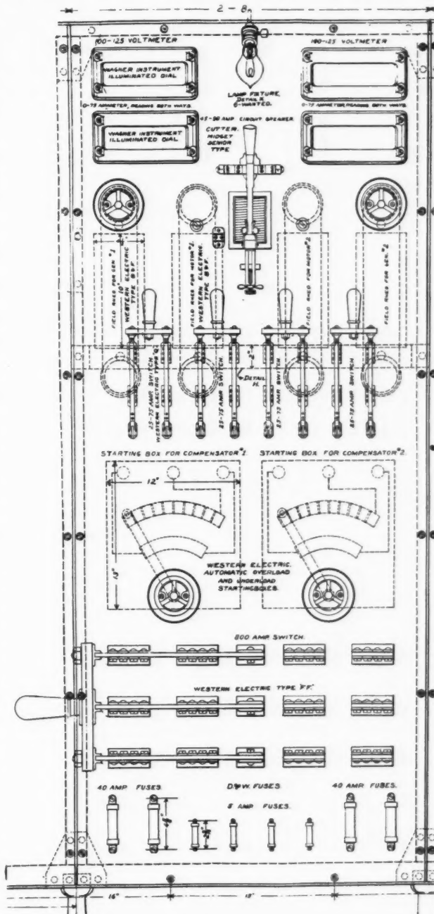
FIG. 7.—COMPENSATOR PANEL.
