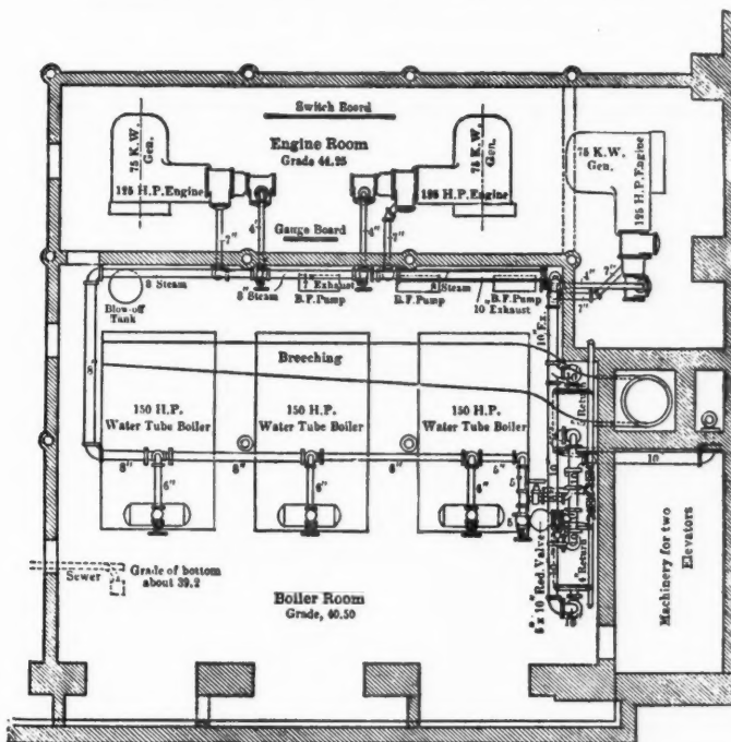
FIG. 2.—PLAN OF BOILER AND ENGINE ROOM.
