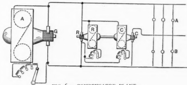
FIG. 6.—COMPENSATOR PLANT.
