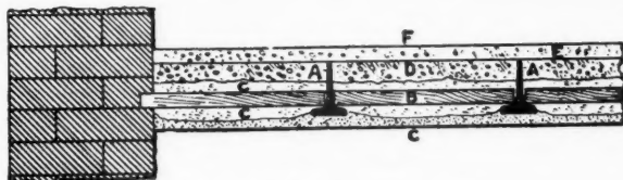
FIG. 2.—FOX &amp; BARRETT'S FLOOR.
