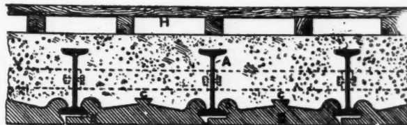
FIG. 5.—SWARBRICK'S FLOOR.
