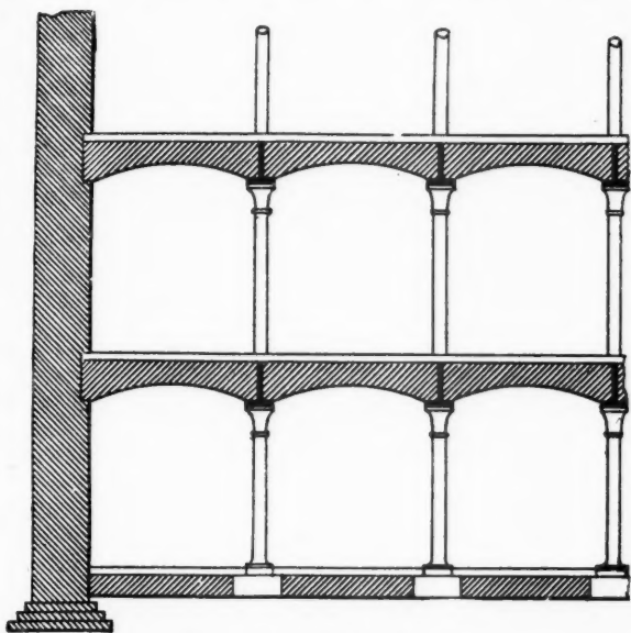
FIG. 1.—FIREPROOF FLOOR, 1801.
