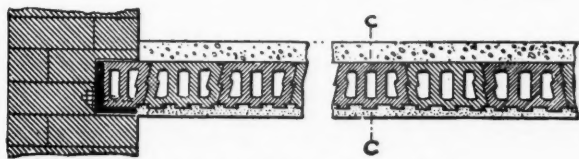
FIG. 3.—SECTION OF BUNNETT'S FLOOR.
