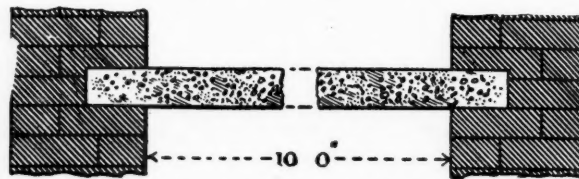
FIG. 9.—SLAB OR PLATE FLOOR.
