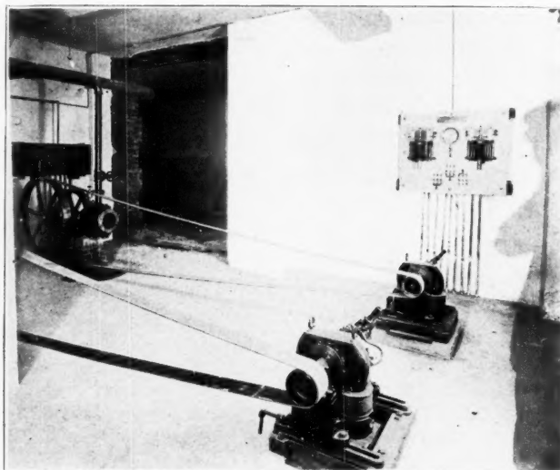
MOTORS CONNECTED WITH EJECTOR PUMPS.
