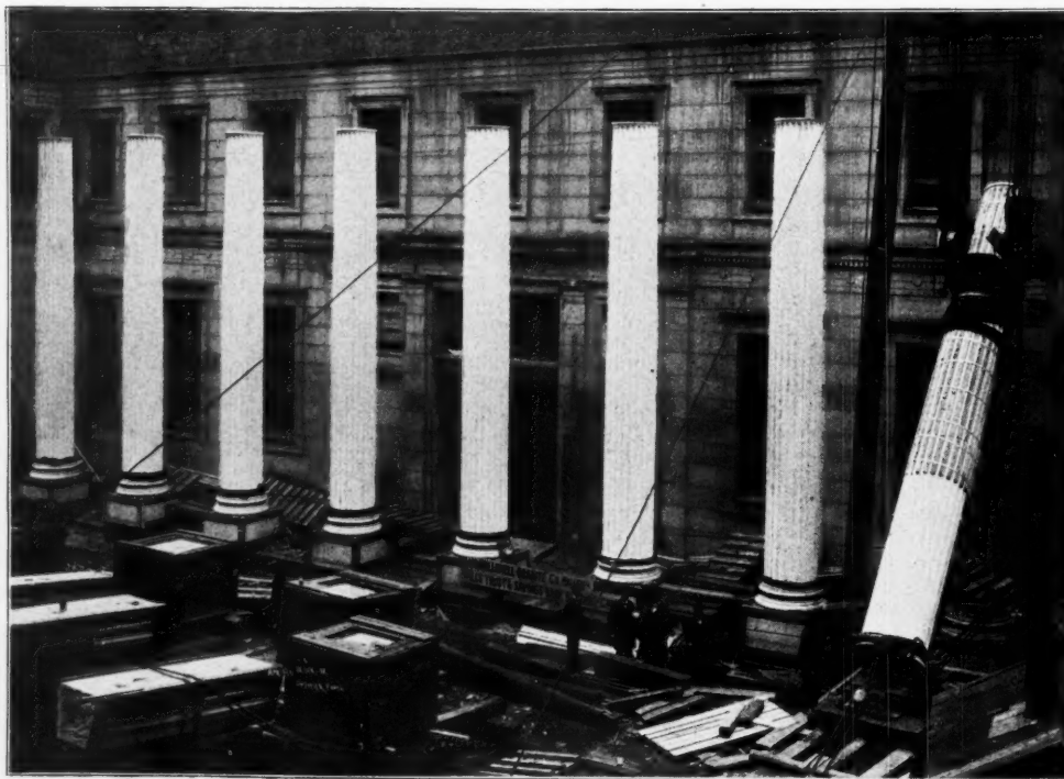
PLACING THE LAST COLUMN.
