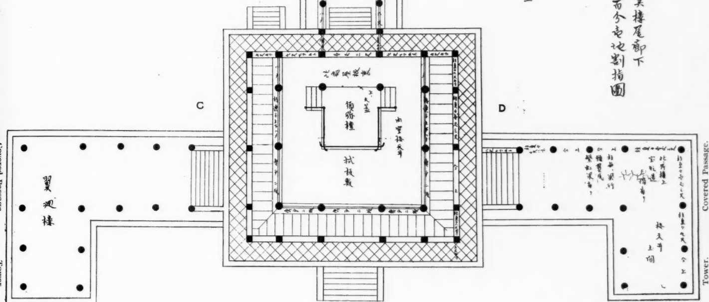
GROUND PLAN. Scale, \frac{1}{2} inch = 1 foot (nearly).
